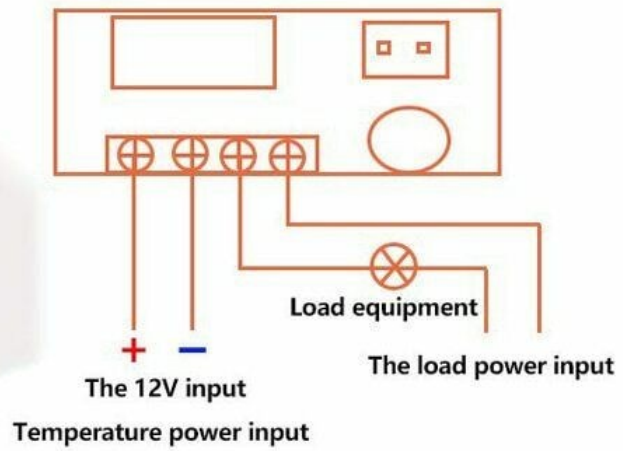
Load and temperature control different power wiring diagram
