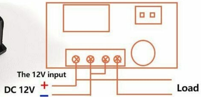
Temperature control and load the 12V cases wiring way
