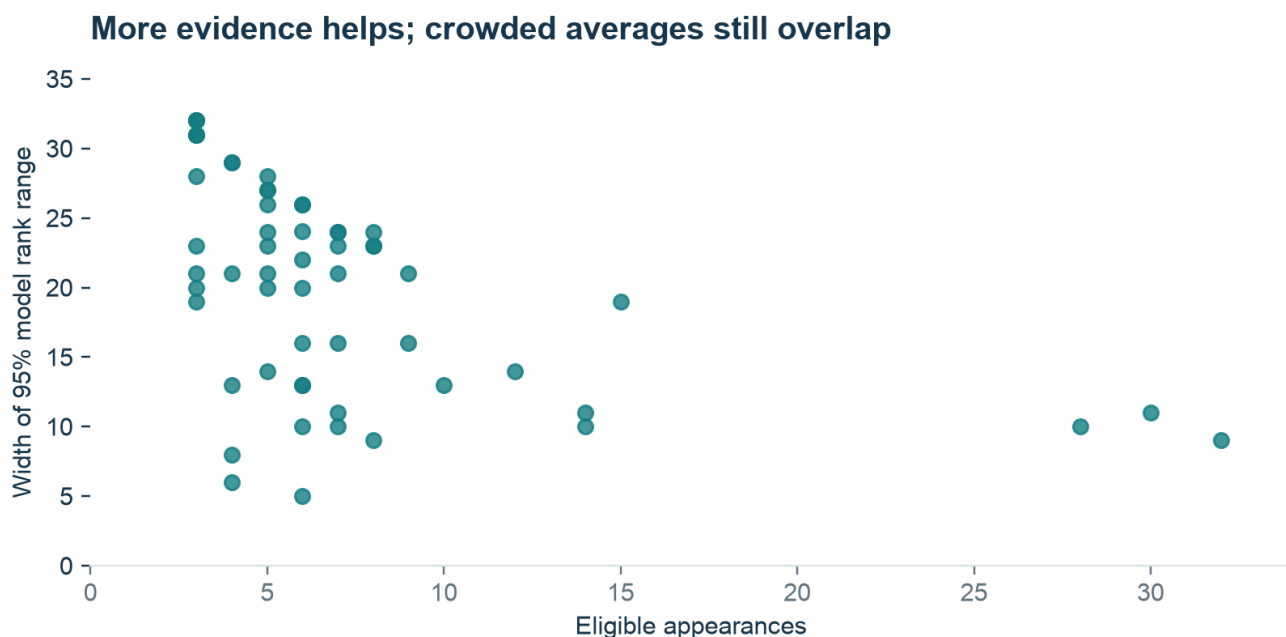
Figure 3. Appearance counts matter, but proximity to other averages and ordinary score variation also affect rank precision.
