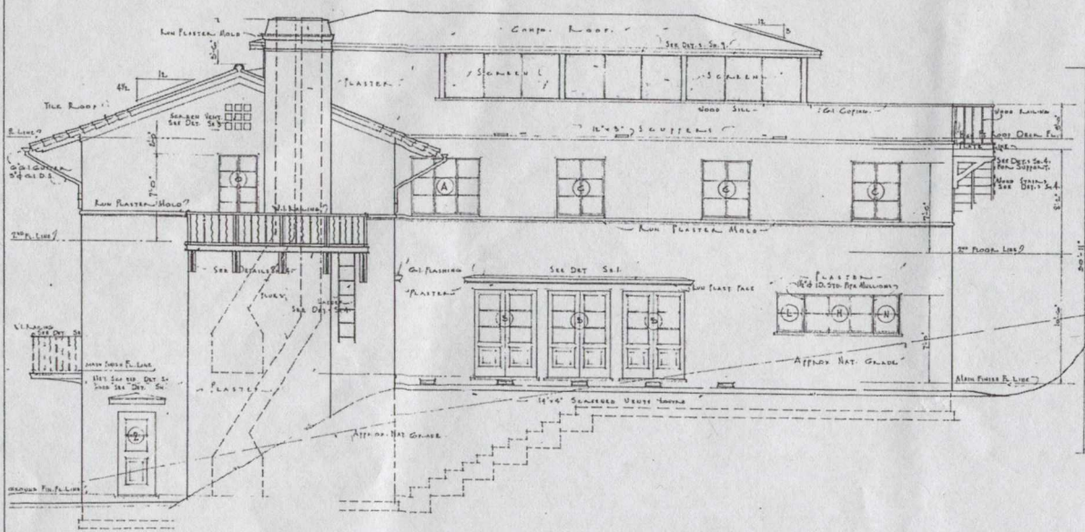
NORTH ELEVATION SCALE 1/4\"/>
