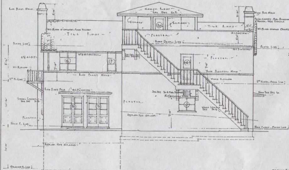
WEST ELEVATION SCALE 1/4\"/>
