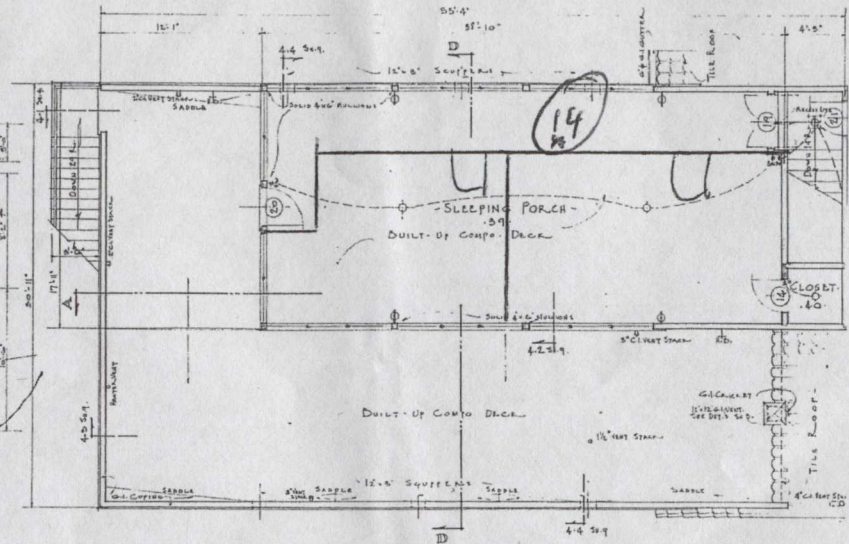
THIRD FLOOR PLAN SCALE 1/4\"/>
