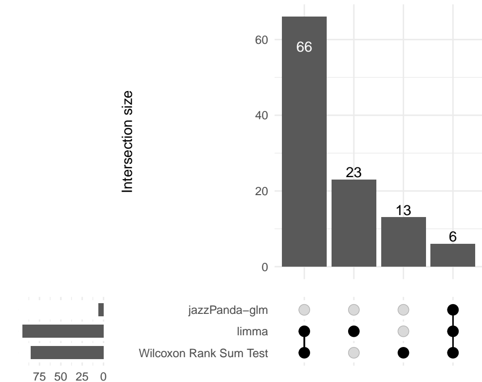
Basal-ciliated epithelium
