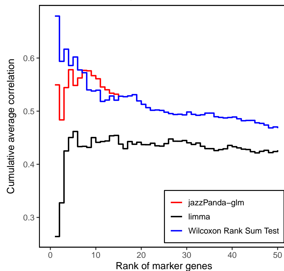
NonNeur_CP_VascStromal
