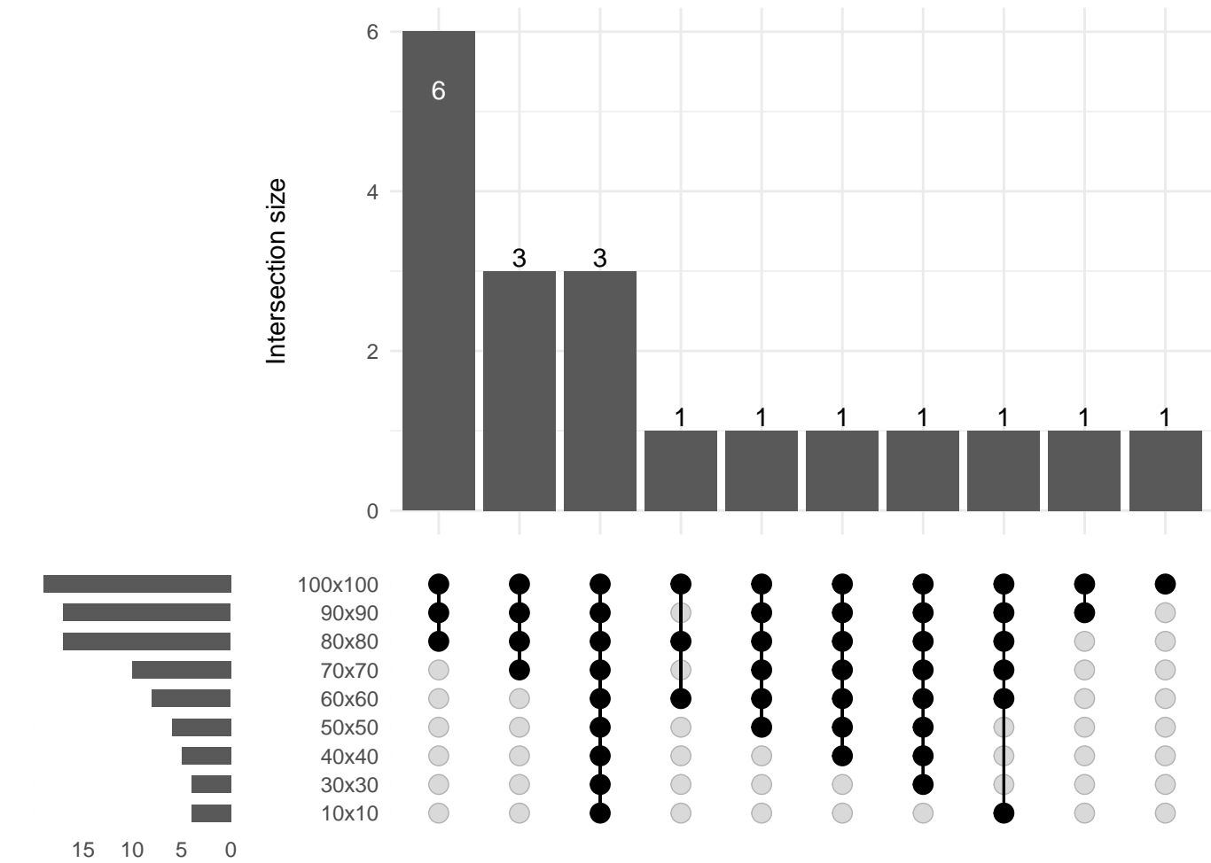
Hep cells
