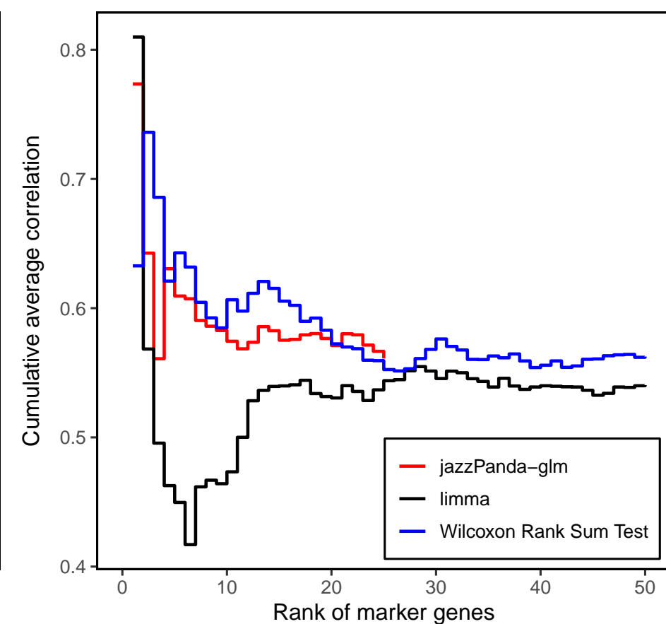
Inh_Striatum_MSN
