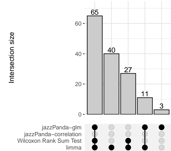
Venous/HEV endothelium
