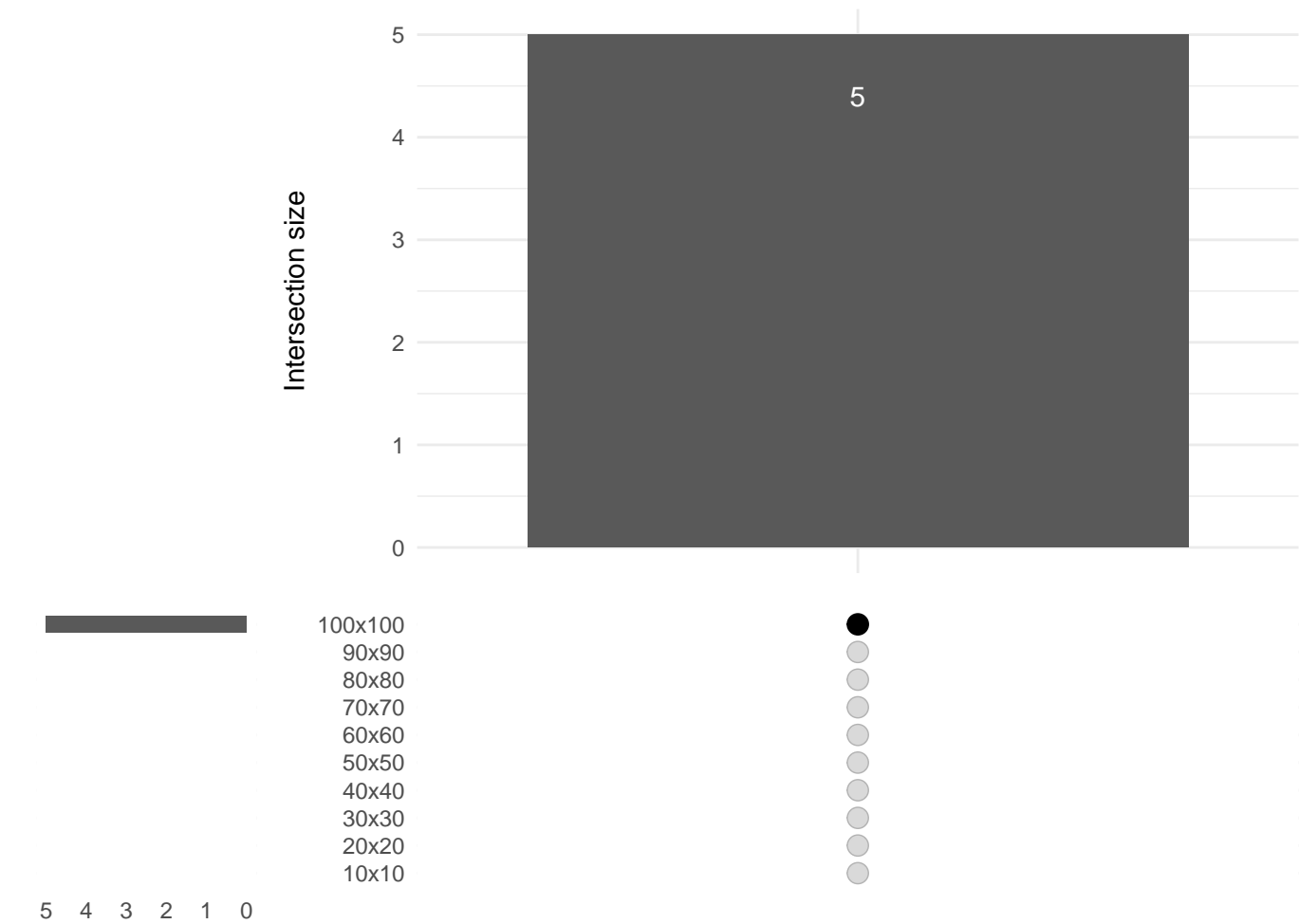
Central.venous.LSECs cells
