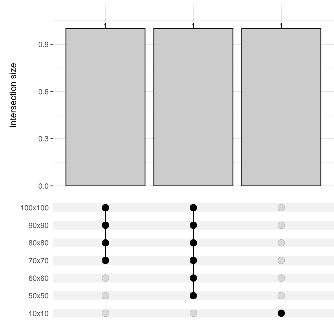
Erthyroid cells
