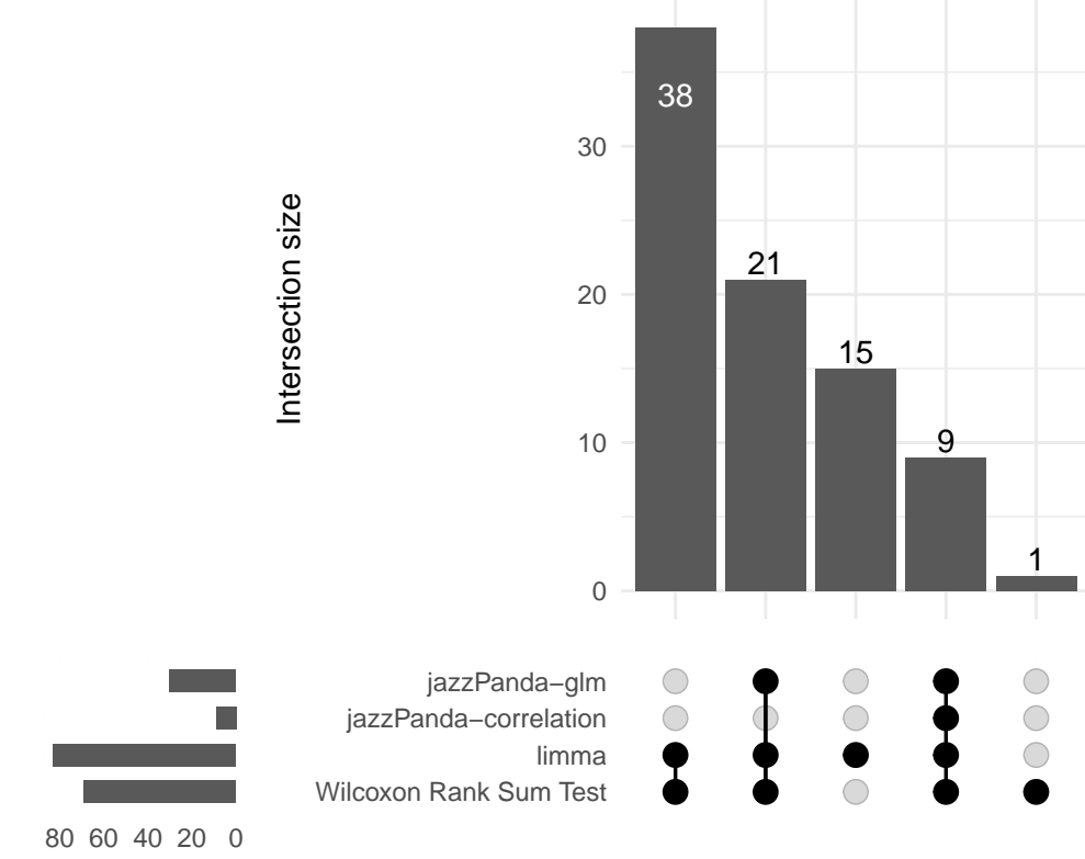
Capillary endothelium
