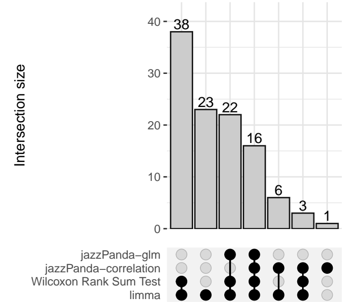
Myofibroblast CAF
