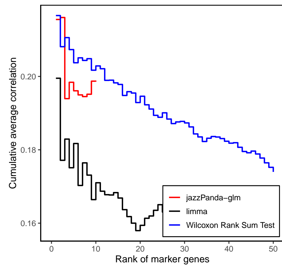
Exc_DG_Granule
