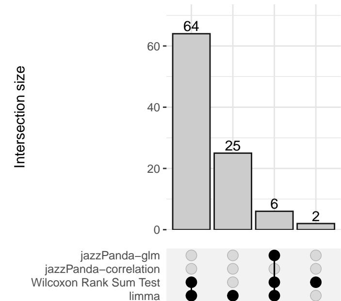
Basal-ciliated epithelium
