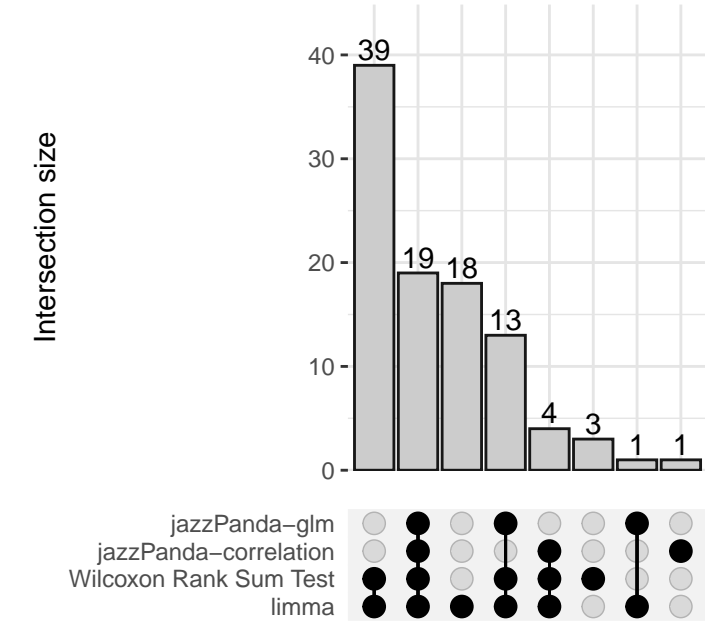
Secretory epithelial
