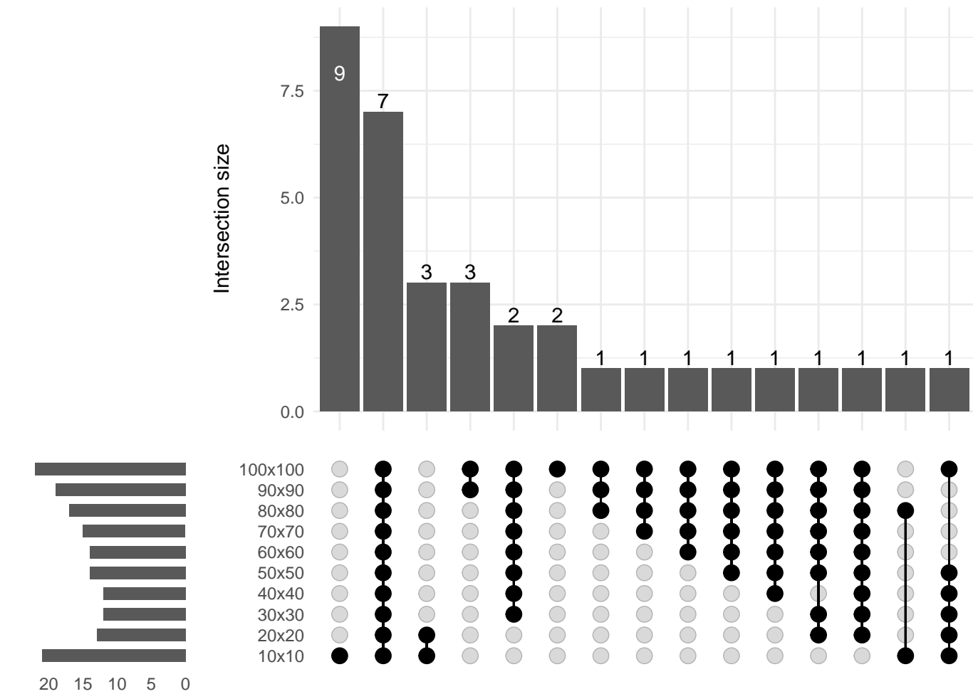
Periportal.LSECs cells
