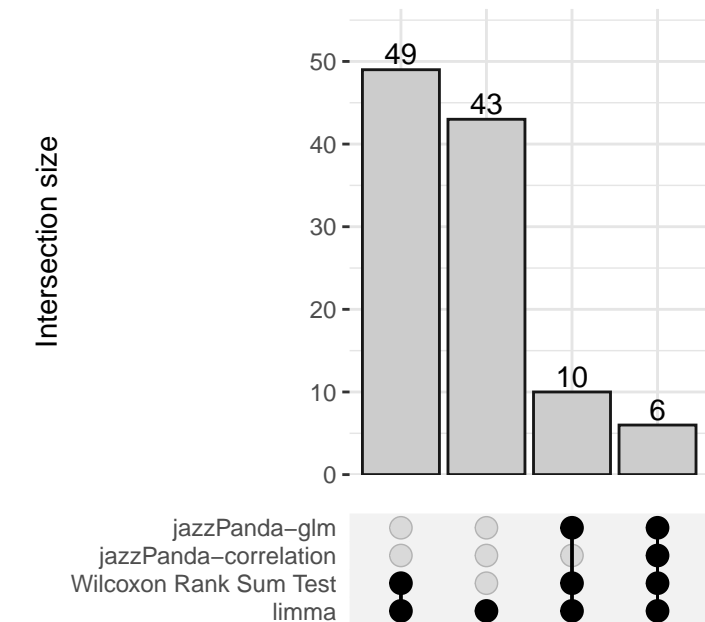
Plasma cell
