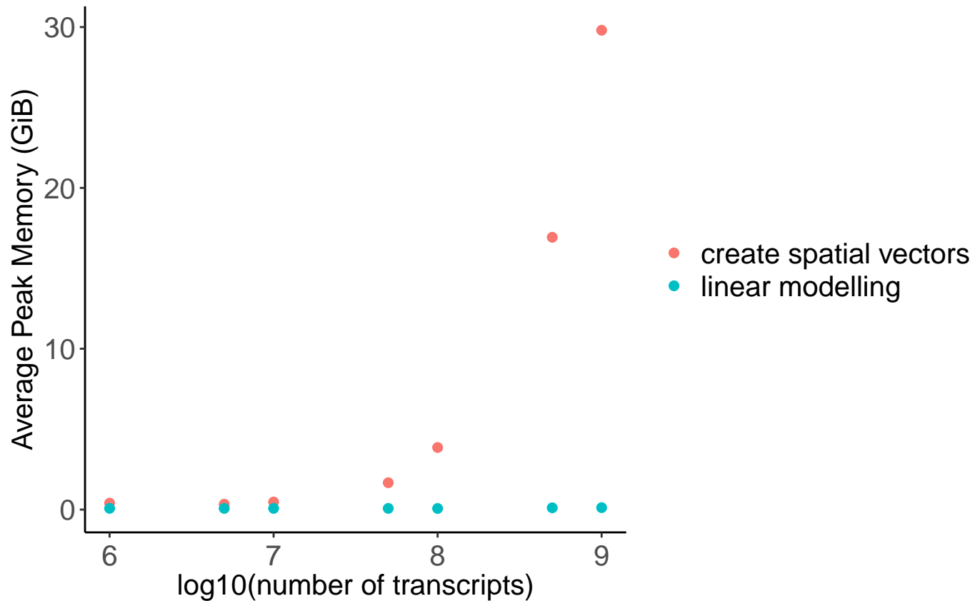
Memory usage
