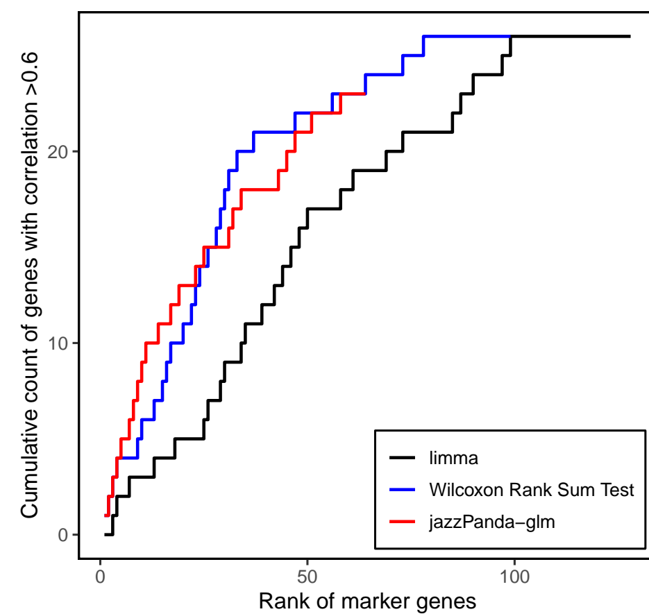
Exc_L6_CTlike
