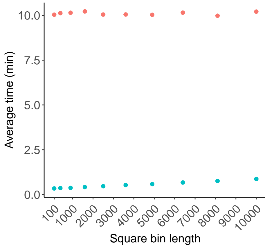
Time usage
