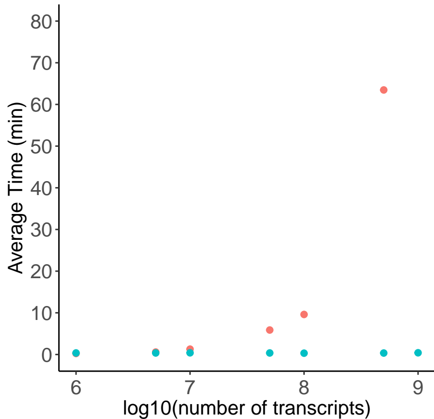
Time usage
