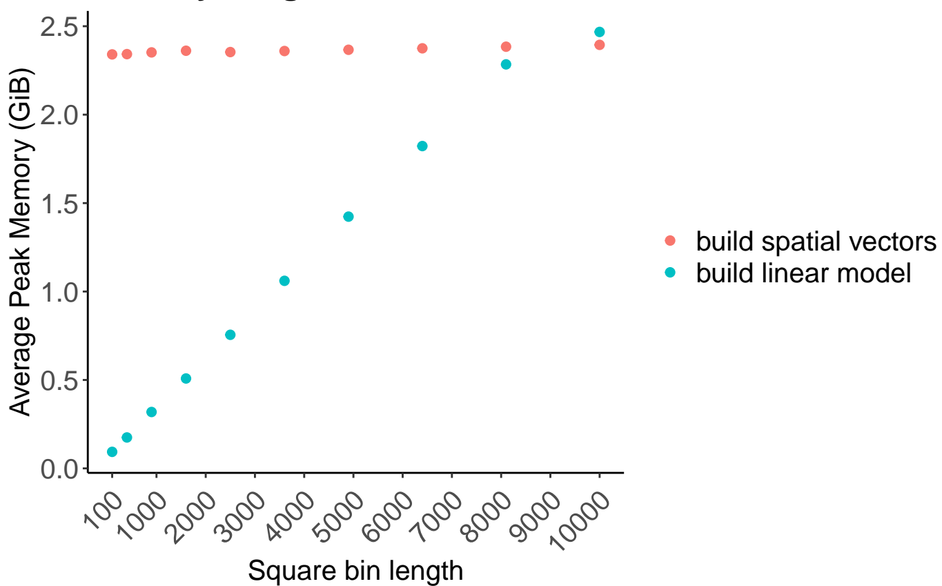
Memory usage
