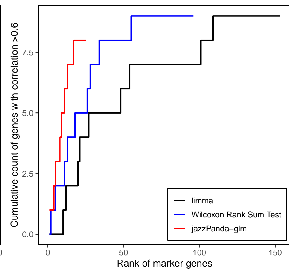
Inh_Striatum_MSN
