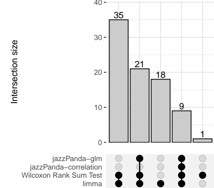
Capillary endothelium
