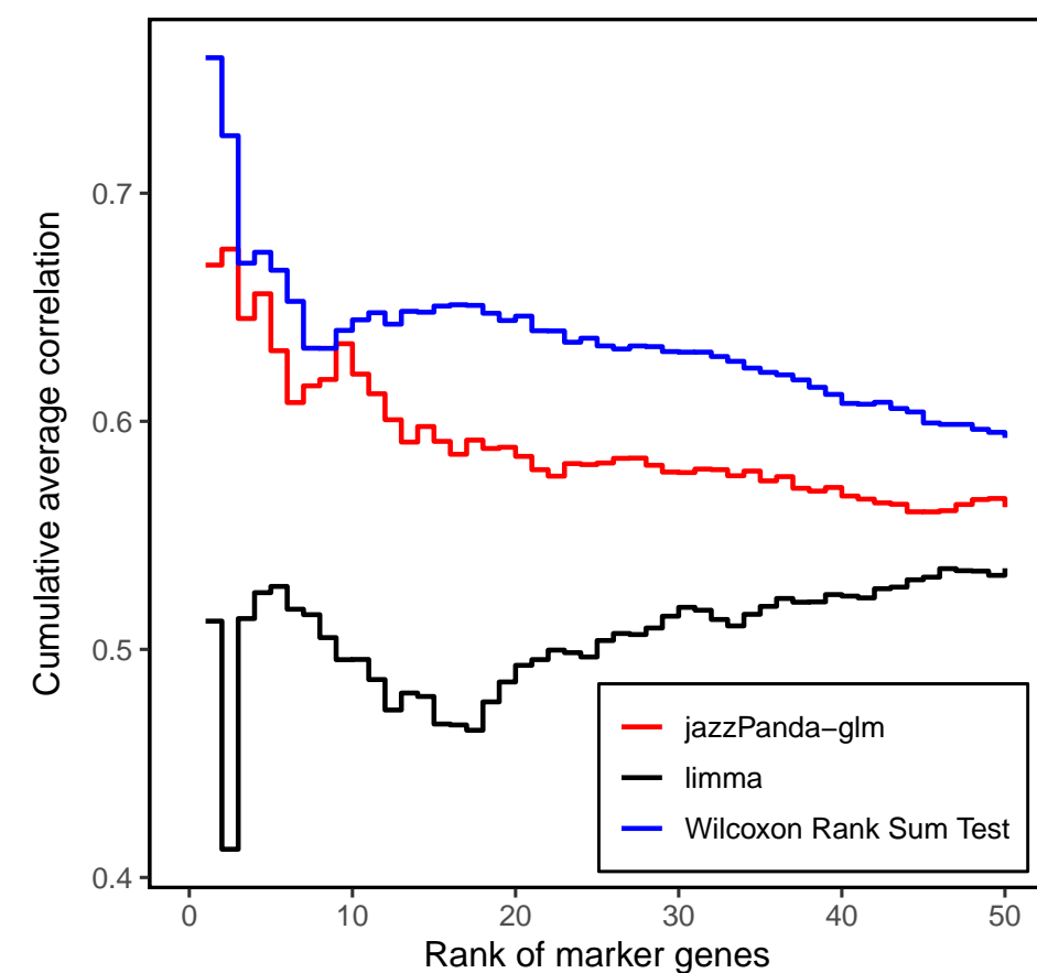
Exc_L6_CTlike
