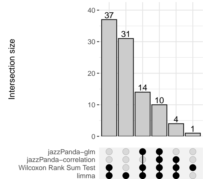
cDC2 / Mono-DC
