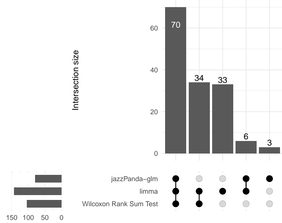
Venous/HEV endothelium
