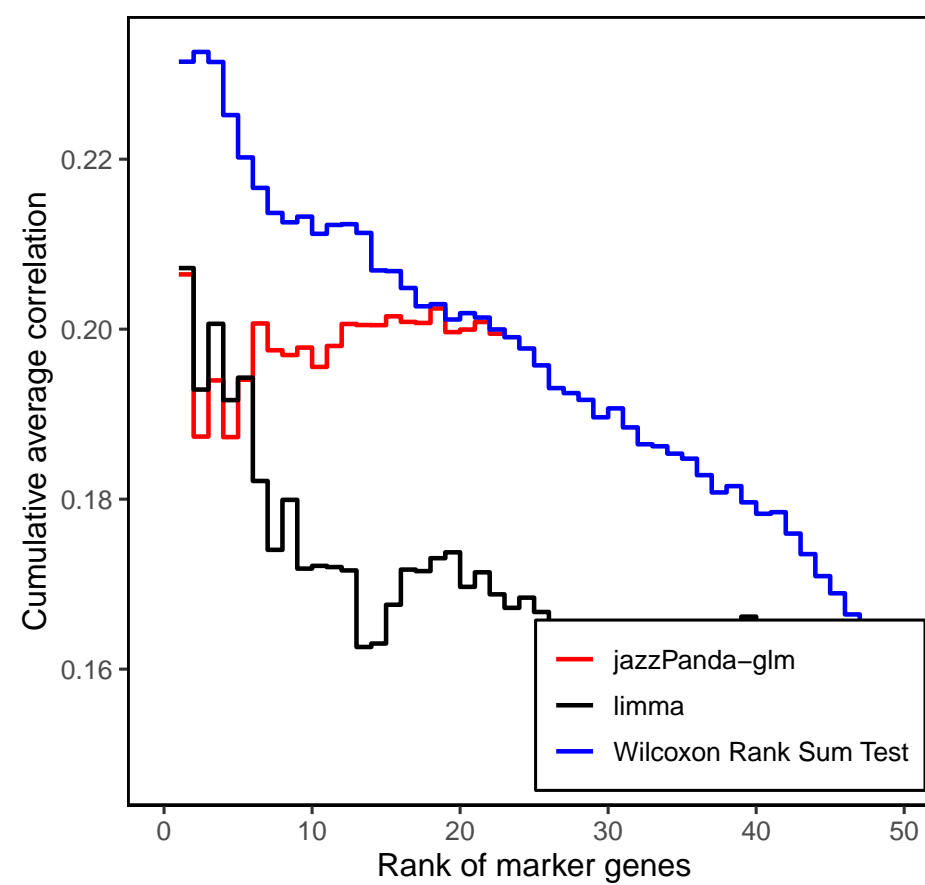
Exc_L6_IT_CC
