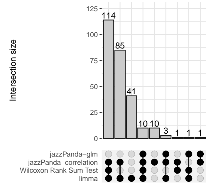
Tcell_Activated
