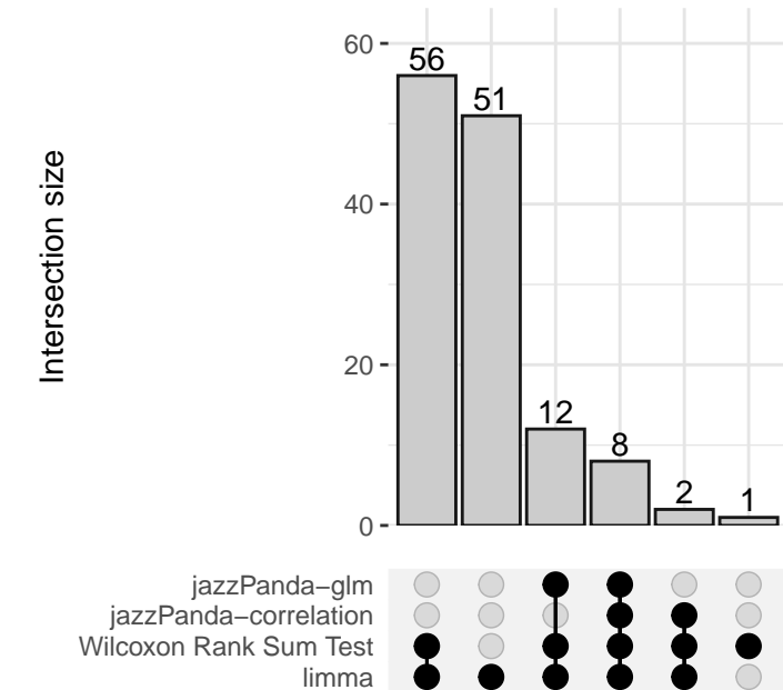
Plasma cell
