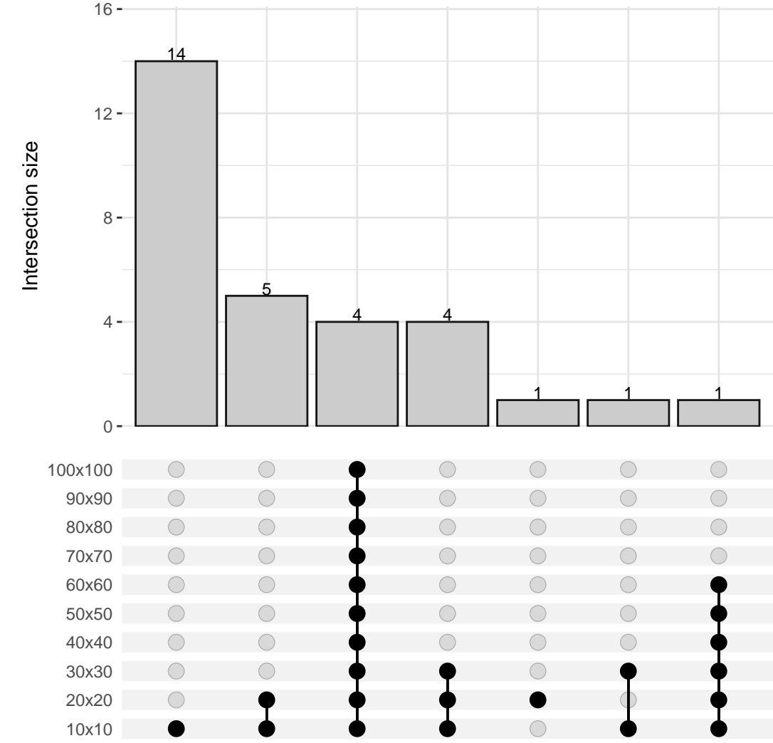
T cells
