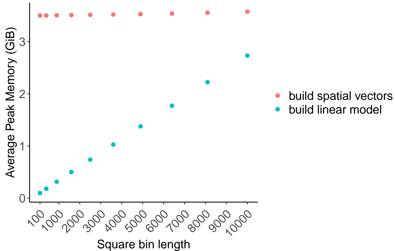
Memory usage
