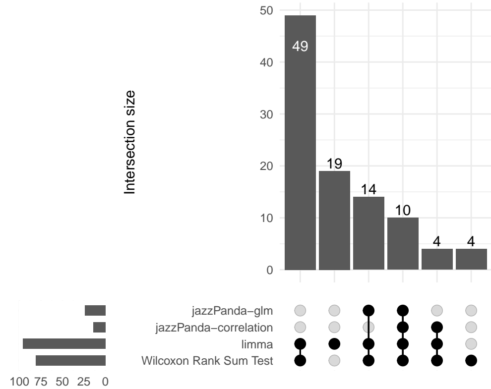
cDC2 / Mono-DC
