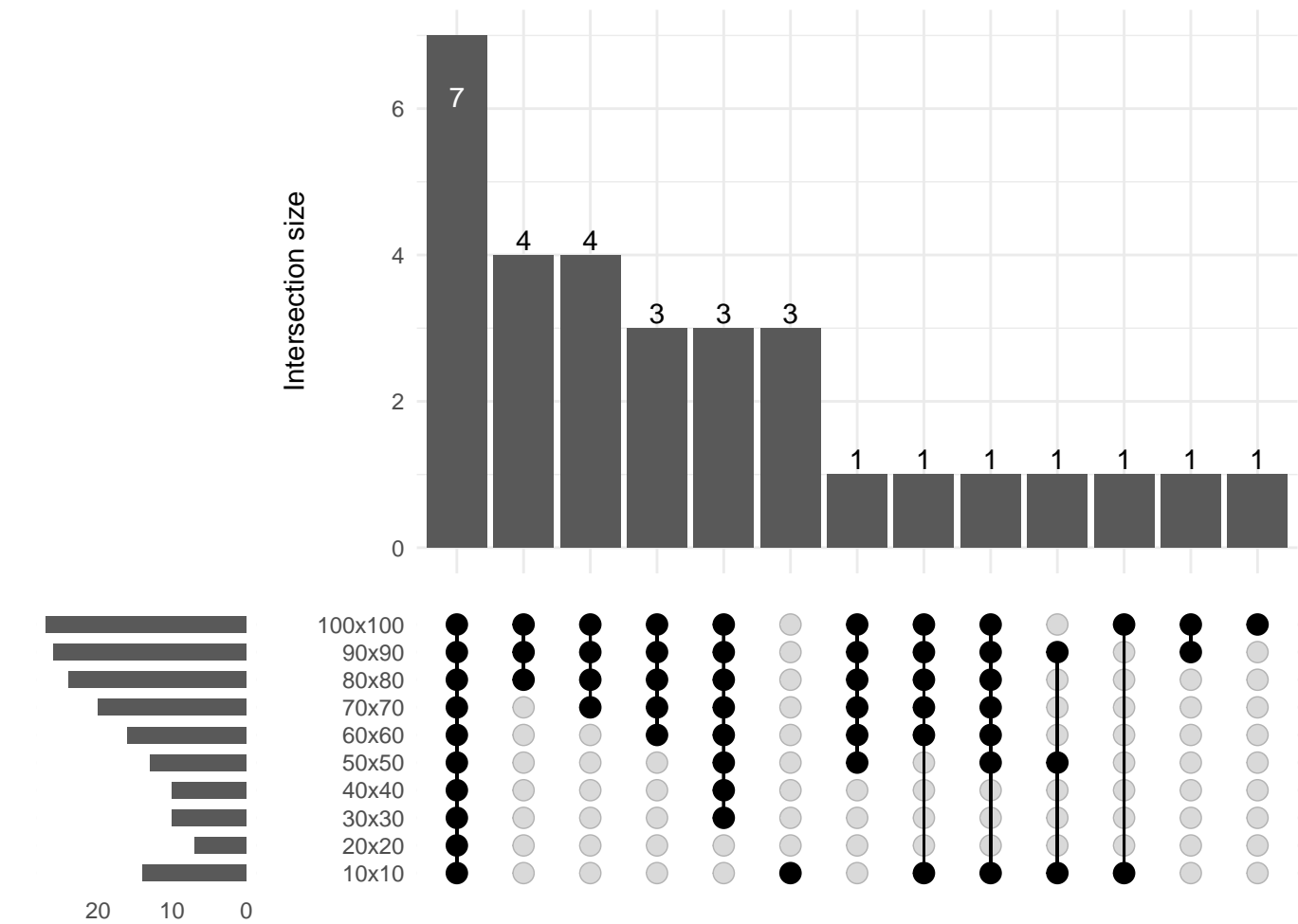
Stellate cells
