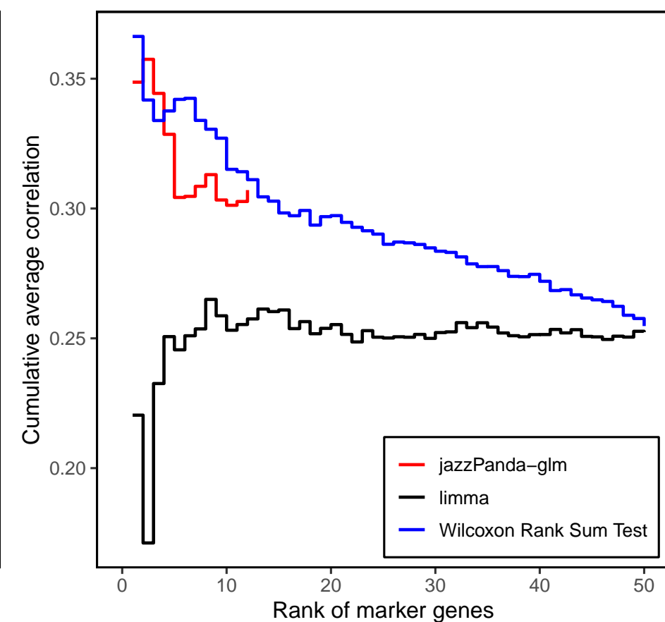
Cholin_ChAT_SNCG
