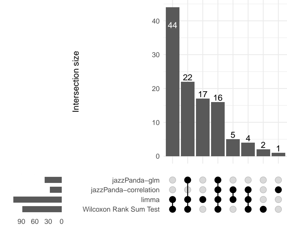
Myofibroblast CAF
