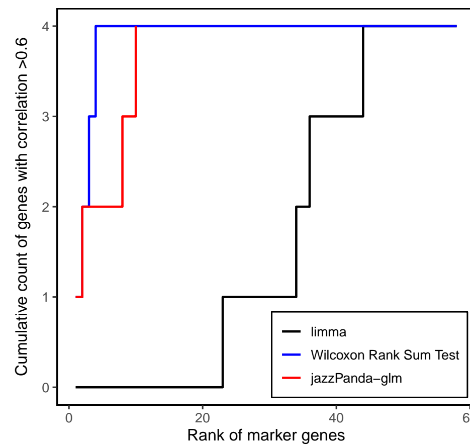
Exc_DG_Granule
