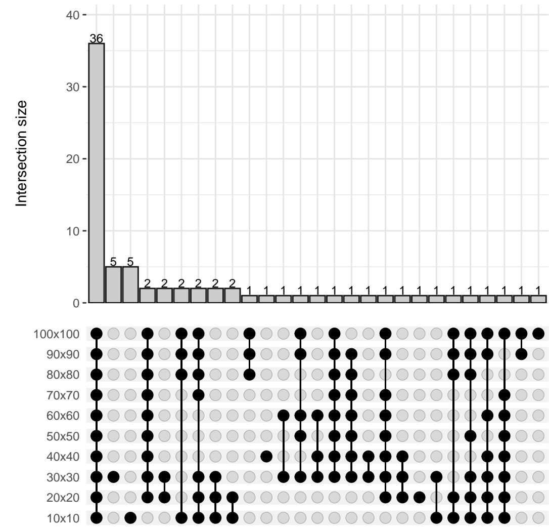
Periportal.LSECs cells
