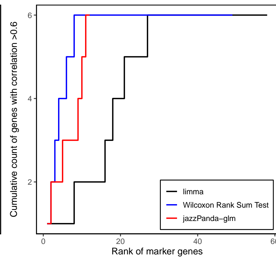
Cholin_ChAT_SNCG
