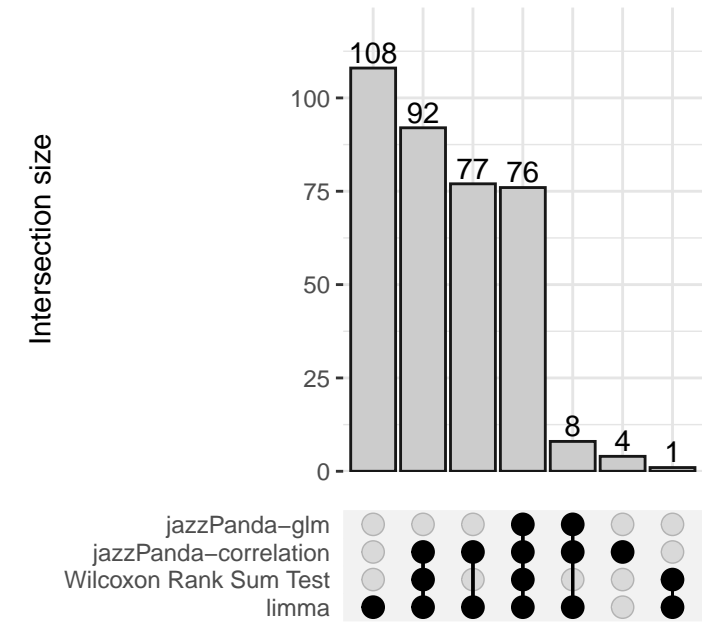
TAM_C1QC
