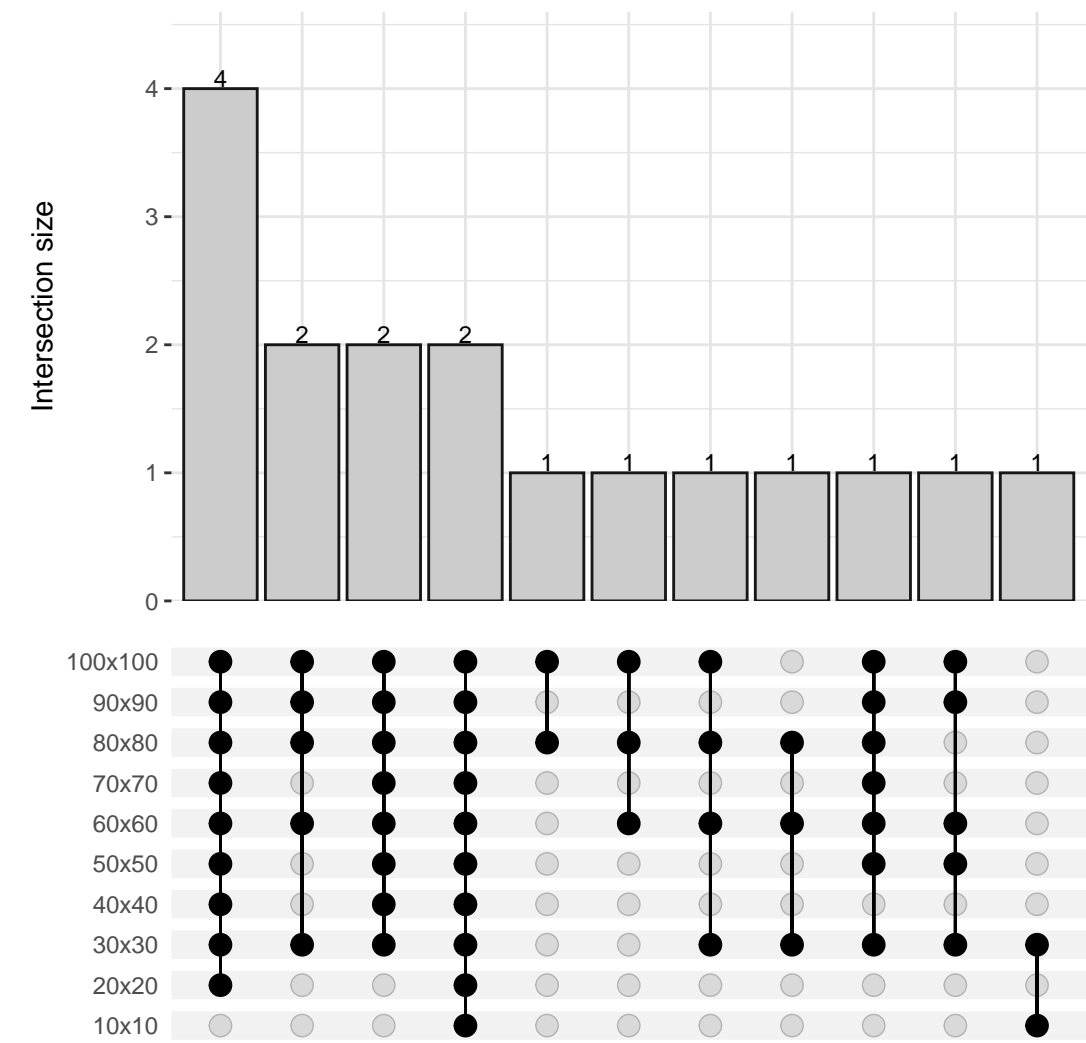
B cells
