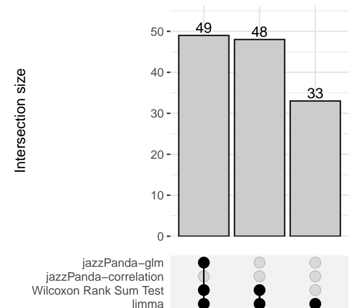
Basal-ciliated epithelium
