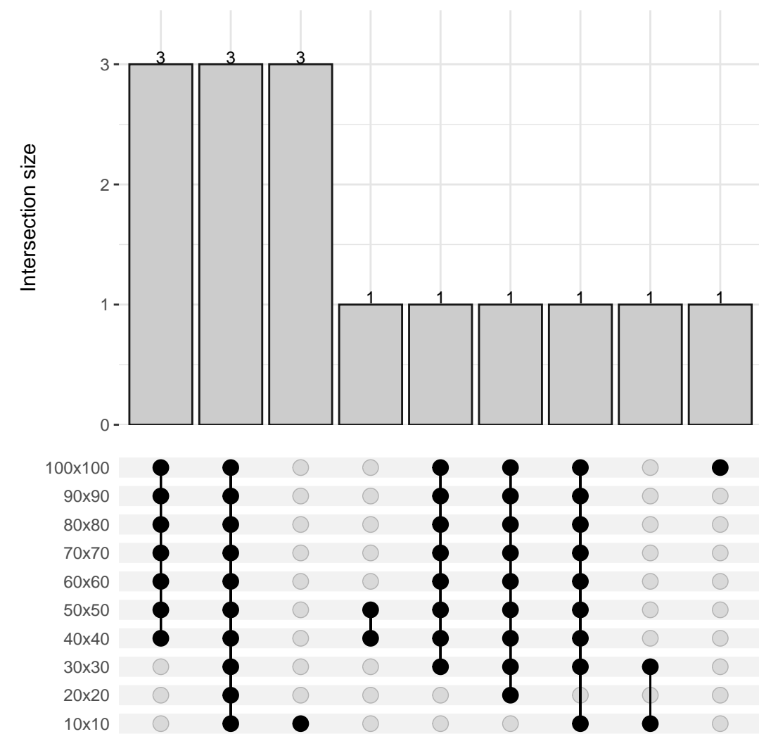
Hep cells
