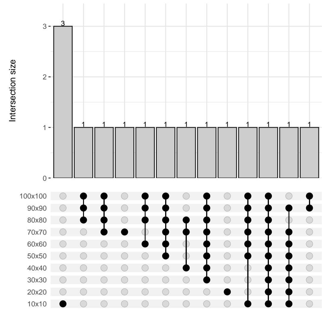
Central.venous.LSECs cells
