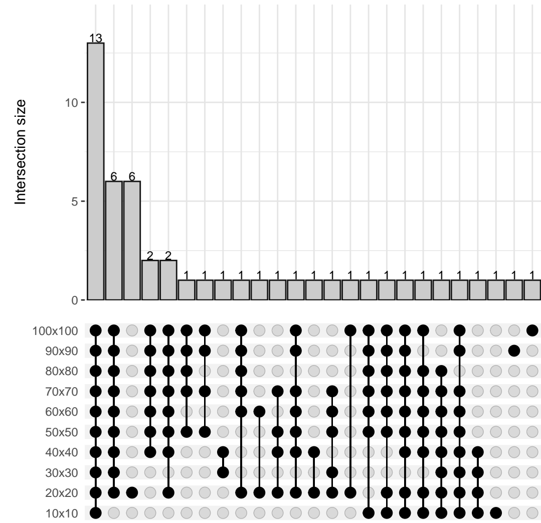
Stellate cells
