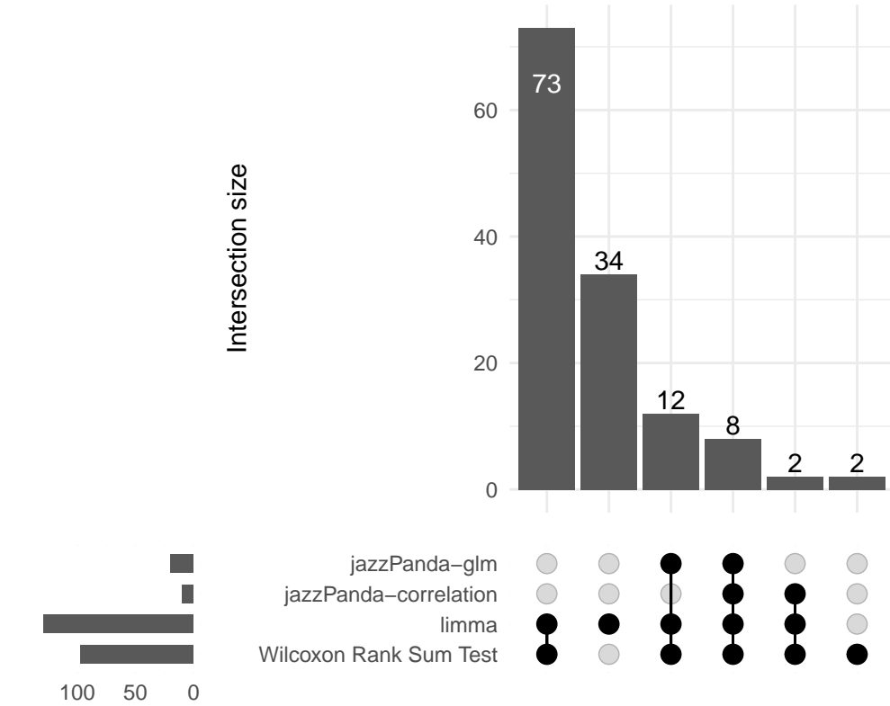
Plasma cell
