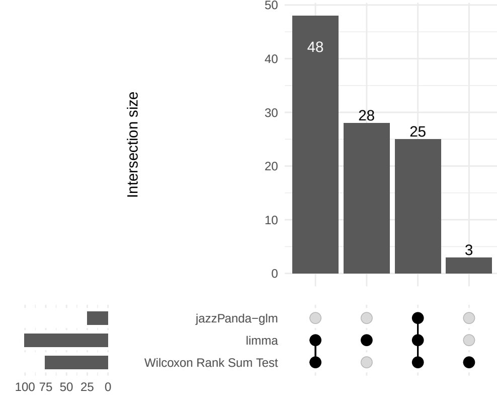
Myoepithelial
