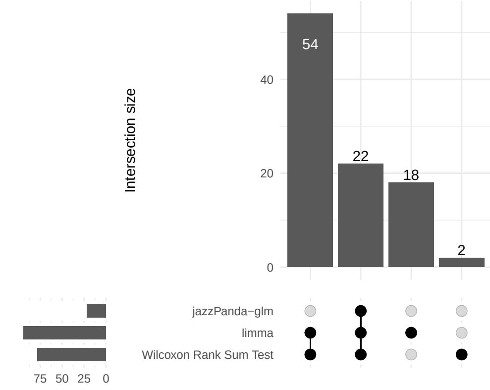
Endothelial
