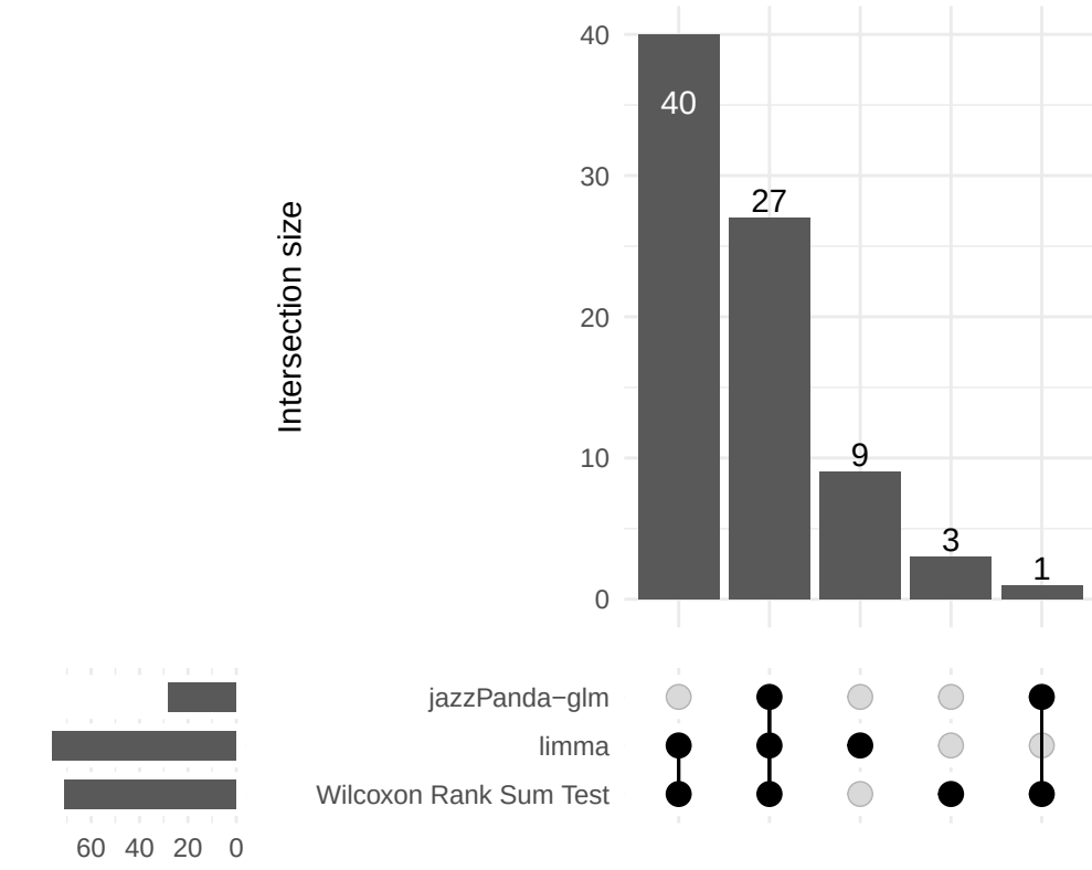
Macrophages
