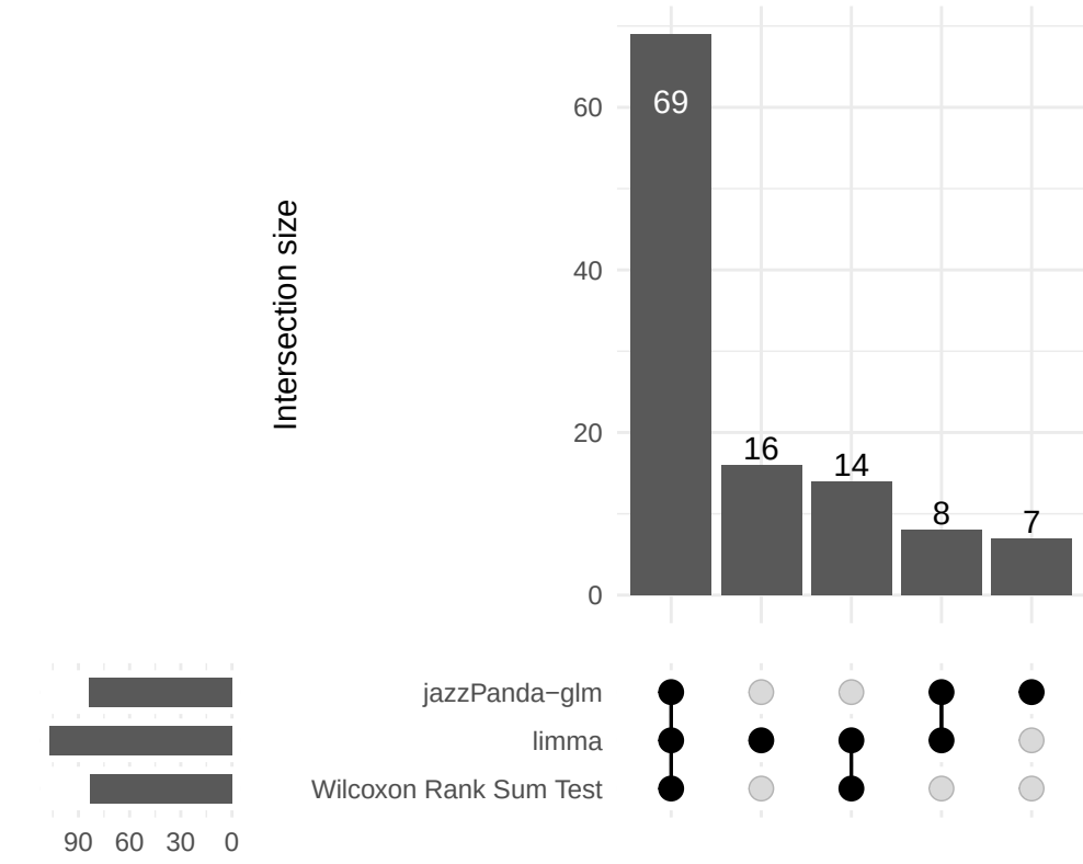
Tumor
