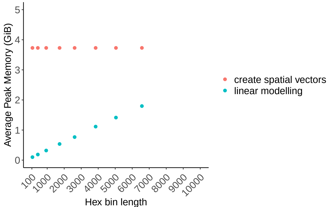
Memory usage
