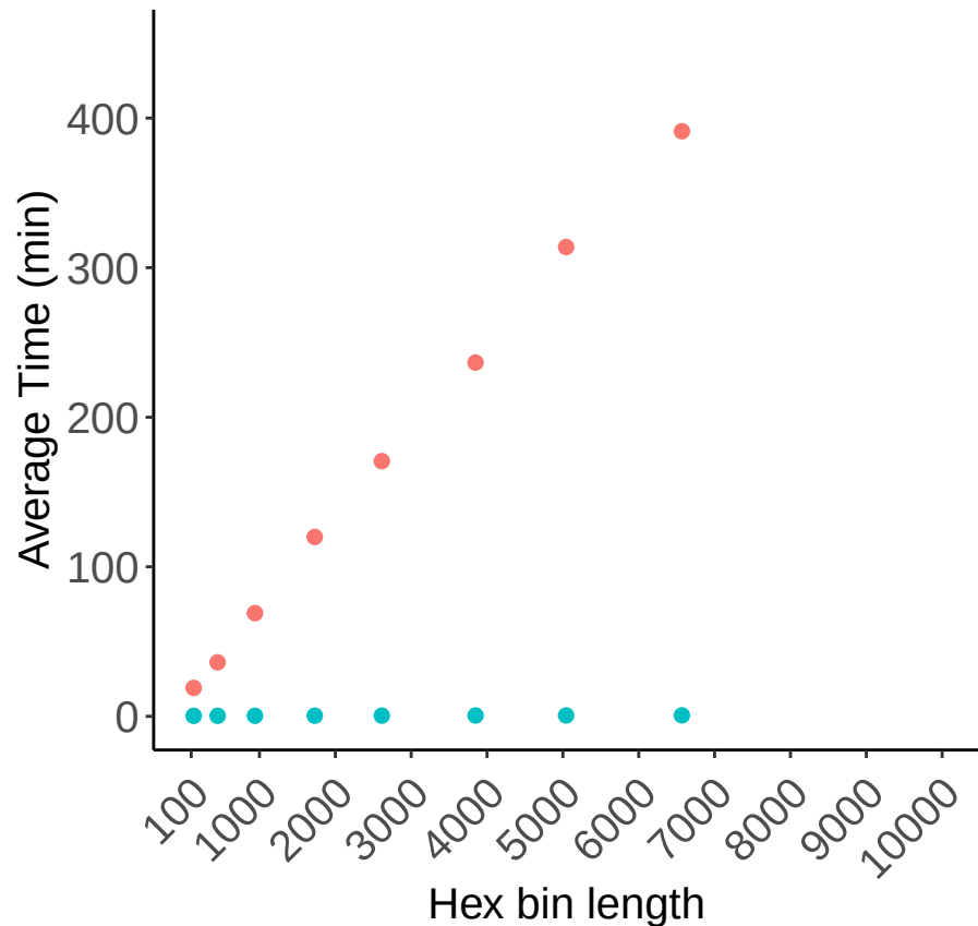
Time usage
