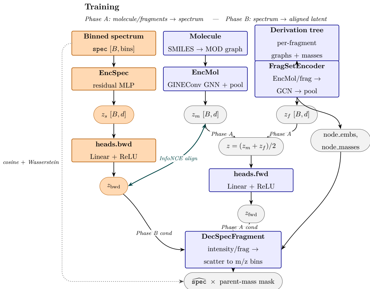
Figure 3.8: Training-time dataflow of the bidirectional framework. Phase A (blue): a molecule graph and its derivation tree are encoded to z_m and z_f , averaged into z_{\text{combined}} = (z_m + z_f)/2 , projected by \text{Head}_{\text{FWD}} , and decoded to \hat{s} by the shared fragment-grounded decoder, which places one intensity per fragment at that fragment’s mass. Phase B (amber): the binned spectrum is encoded to z_{\text{spec}} and projected by \text{Head}_{\text{BWD}} to z_{\text{bwd}} , which is aligned to the molecular latent z_m by an InfoNCE objective and conditions the same decoder. Dotted edges denote spectrum-reconstruction losses (cosine and Wasserstein); the full set of loss terms is listed in Table 3.2.
