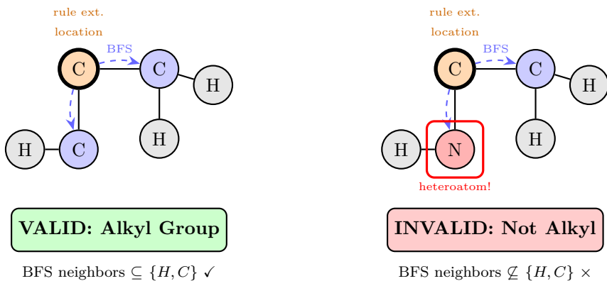
Figure 3.5: Alkyl check predicate formulated as a constrained path traversal. Starting from the rule extension location, a breadth-first search (BFS) is performed over the local molecular graph to verify that all reachable neighboring atoms belong to the set \{C, H\} . A matched substructure is accepted as an alkyl group if only carbon and hydrogen atoms are encountered (left), whereas the presence of a heteroatom such as nitrogen causes the predicate to fail (right).
