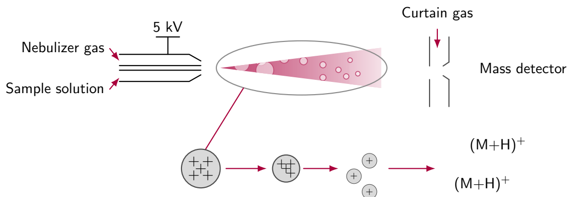
Figure 2.3: Schematic illustration of the electrospray ionization (ESI) process. A sample solution is dispersed by nebulizer gas and subjected to a high electric potential, producing a spray of charged droplets. Progressive solvent evaporation and droplet fission lead to the formation of gas-phase ions, which are transferred through the interface region into the mass detector. The figure highlights the transition from charged droplets to molecular ions, exemplified here by protonated species (M + H)^+ .
