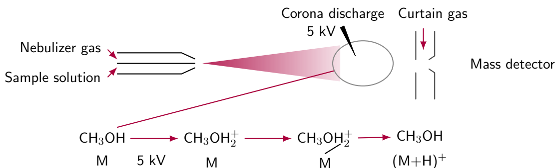
Figure 2.4: Schematic illustration of atmospheric pressure chemical ionization (APCI). The sample solution is nebulized and vaporized, and a corona discharge operated at high voltage generates reagent ions from the solvent. In the example shown, protonated ions transfer a proton to the analyte molecule M , forming the protonated molecular ion (M + H)^+ , which is then introduced through the interface region into the mass detector.
