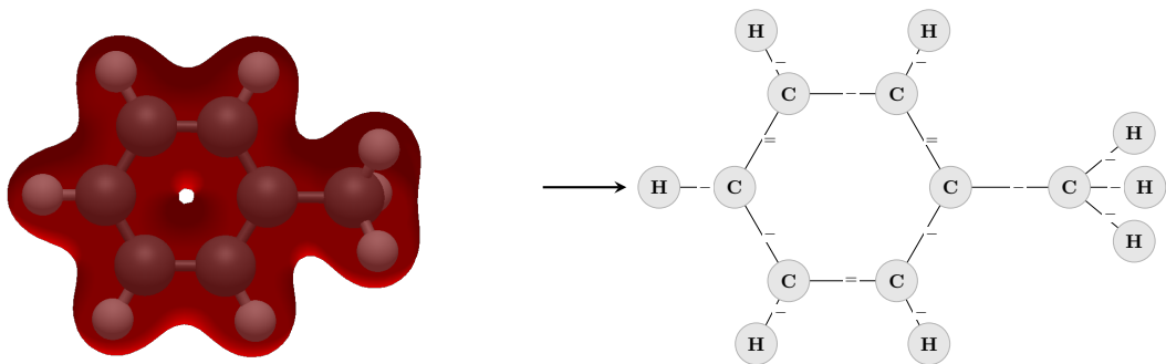
Figure 2.7: Toluene on the left depicted as a quantum-mechanical model with 3D coordinates and electron density, and on the right as a molecular graph abstraction. The graph captures the connectivity of atoms (vertices) and bonds (edges) while abstracting away geometric and electronic details.
