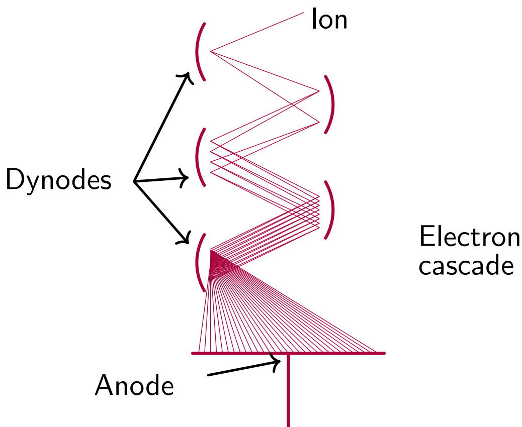
Figure 2.6: Schematic illustration of an electron multiplier (EM) detector. An incoming ion strikes the first dynode, causing the emission of secondary electrons. These electrons are then accelerated to subsequent dynodes, where they generate additional electrons in a cascading effect. After multiple stages, this results in a significant amplification of the original ion signal, producing a measurable current pulse that can be digitized and recorded as part of the mass spectrum.
