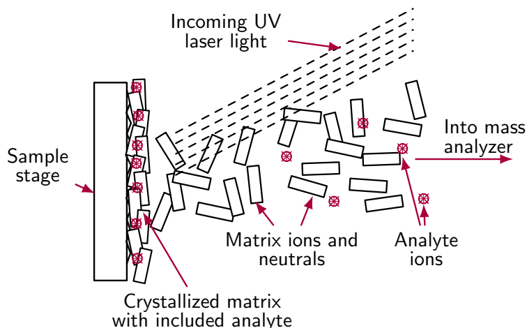
Figure 2.5: Schematic illustration of matrix-assisted laser desorption/ionization (MALDI). A crystallized matrix containing embedded analyte molecules is irradiated with UV laser light at the sample stage, leading to desorption and ionization of matrix and analyte species. During plume formation, matrix ions and neutrals promote the formation of analyte ions, which are subsequently transferred into the mass analyzer.
