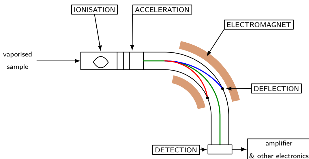
Figure 2.2: Simplified schematic of the measurement principle in a magnetic sector mass spectrometer. Following sample introduction, ionisation and acceleration generate an ion beam that is separated in the magnetic field by deflection that depends on m/z . The separated ions are then detected and transformed into an electrical signal for further processing. [18]
