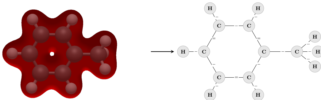
Figure 2.12: Toluene on the left depicted as a quantum-mechanical model with 3D coordinates and electron density, and on the right as a molecular graph abstraction. The graph captures the connectivity of atoms (vertices) and bonds (edges) while abstracting away geometric and electronic details.
