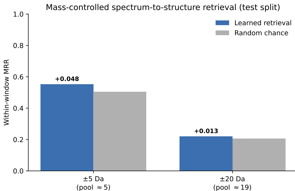
Figure 4.2: Spectrum-to-structure retrieval on held-out test molecules, with precursor mass taken into account. For each mass window ( \pm 5 and \pm 20 Da around the query’s true mass), the learned encoder retrieval MRR is shown next to the analytic random-chance MRR for a pool of the same size. A bar standing above its chance reference indicates structural signal that mass alone cannot explain, since mass is approximately constant inside the window. This is the decisive test for structural signal: uncontrolled retrieval quality can be explained by mass alone, whereas here the model retains a positive margin over chance once mass is controlled for.
