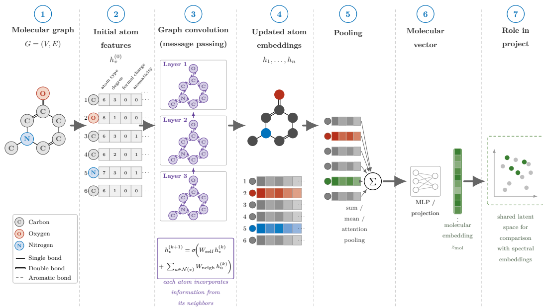
Figure 2.15: Starting from the molecular graph G = (V, E) in column 1 , where atoms form the nodes and bonds form the edges, each atom is initialized with a feature vector in column 2 that encodes local chemical properties such as atom type, degree, formal charge, and aromaticity. Through repeated graph-convolution/message-passing layers in column 3 , these atom representations are updated by aggregating information from neighboring atoms, yielding the context-aware atom embeddings shown in column 4 . These embeddings are then pooled over all atoms in column 5 to obtain a fixed-length molecular representation, which is projected in column 6 into the shared latent space as the molecular embedding z_{\text{mol}} . As indicated in column 7 , this vector can subsequently be compared with spectral embeddings for molecule-spectrum alignment. The atom features shown here (atom type, degree, formal charge, aromaticity) are a generic illustration of typical GNN inputs; the specific node-feature set used in this work—a one-hot element encoding together with formal charge, radical state, degree, aromaticity, and incident bond order—is defined in Section 3.2.1.
