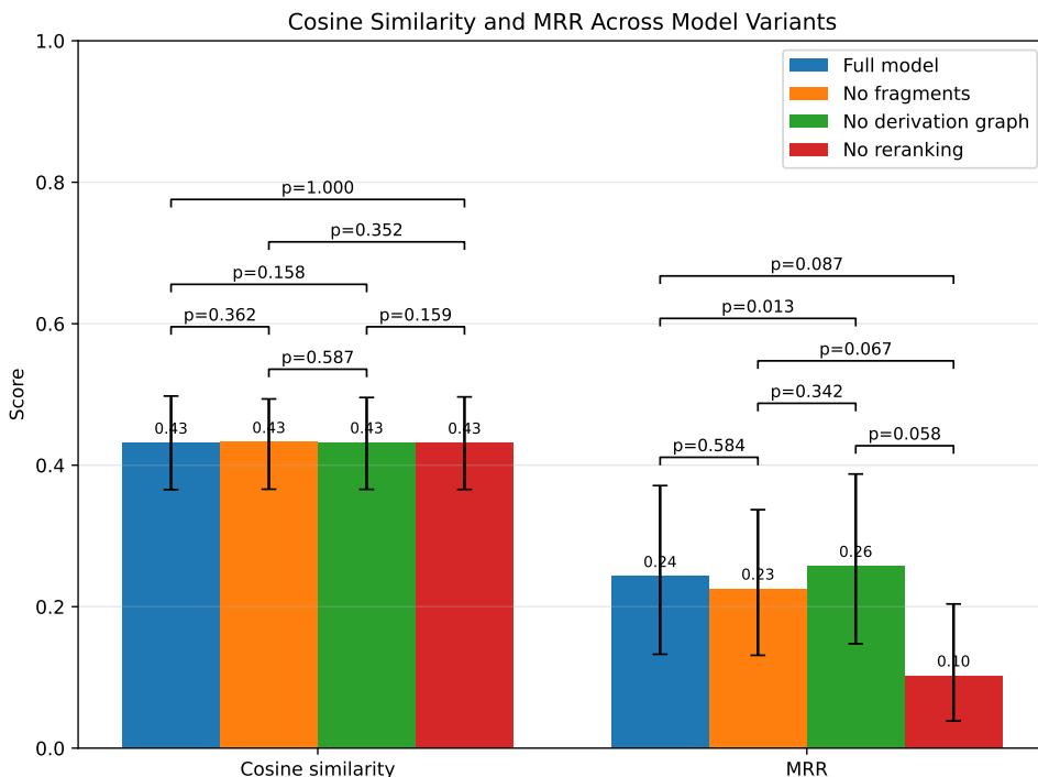
Figure 4.3: Ablation of three pipeline components (fragments, derivation graph, and reranker) against the full model. Cosine similarity measures how similar the query is to the correct target, averaged over all queries; MRR is the mean reciprocal rank of the ground-truth target. Error bars show 95% bootstrap confidence intervals (5000 query resamples). Brackets indicate pairwise p-values from paired randomization tests computed separately for each metric. For cosine similarity , all variants are nearly identical ( \approx 0.43 ) and no pairwise difference is statistically significant, so forward reconstruction is insensitive to the ablations. For MRR , removing reranking lowers the full-set score from 0.24 to 0.10 (Full vs. no-reranking, p \approx 0.087 ), whereas the fragment and derivation-graph ablations do not differ significantly from the full model. As discussed in the text, this full-set MRR is dominated by precursor mass, so the reranking effect shown here reflects mass-consistency filtering rather than learned spectral shape.
