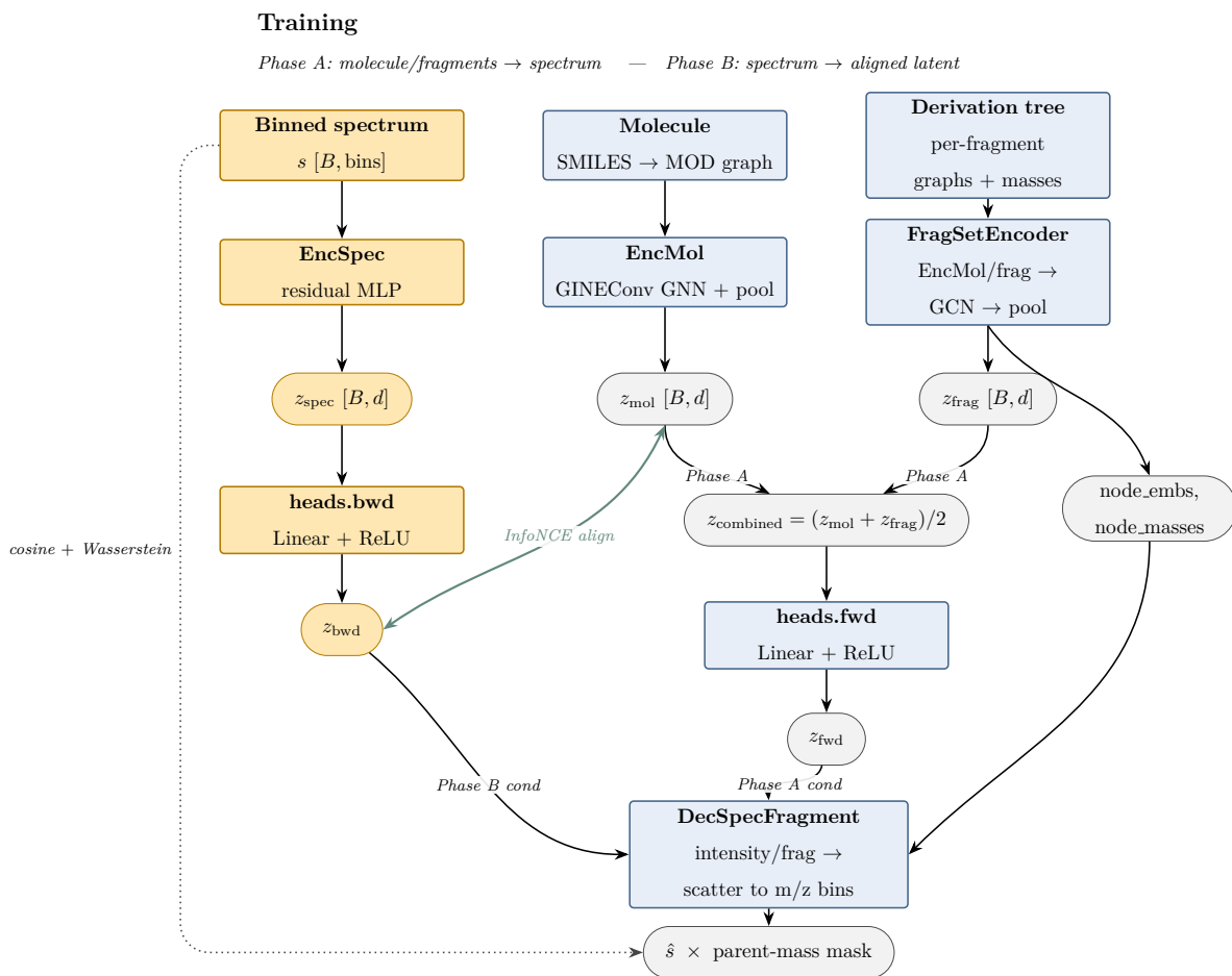
Figure 3.8: Training-time dataflow of the bidirectional framework. Phase A (blue): a molecule graph and its derivation tree are encoded to z_{\text{mol}} and z_{\text{frag}} , averaged into z_{\text{combined}} = (z_{\text{mol}} + z_{\text{frag}})/2 , projected by \text{Head}_{\text{FWD}} , and decoded to \hat{s} by the shared fragment-grounded decoder, which places one intensity per fragment at that fragment’s mass. Phase B (amber): the binned spectrum is encoded to z_{\text{spec}} and projected by \text{Head}_{\text{BWD}} to z_{\text{bwd}} , which is aligned to the molecular latent z_{\text{mol}} by an InfoNCE objective and conditions the same decoder. Dotted edges denote spectrum-reconstruction losses (cosine and Wasserstein); the full set of loss terms is listed in Table 3.2.
