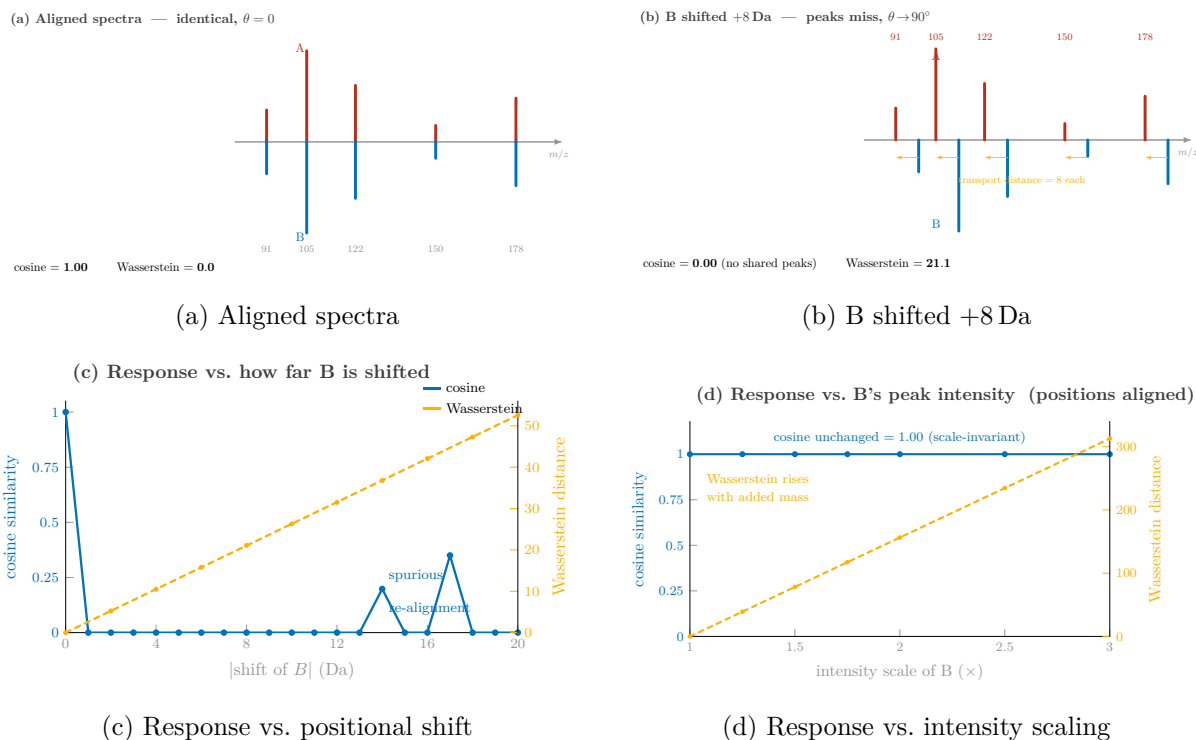
Figure 2.11: Spectrum A (red) is plotted upward and spectrum B (blue) mirrored downward on a shared m/z axis with non-uniformly spaced peaks.
