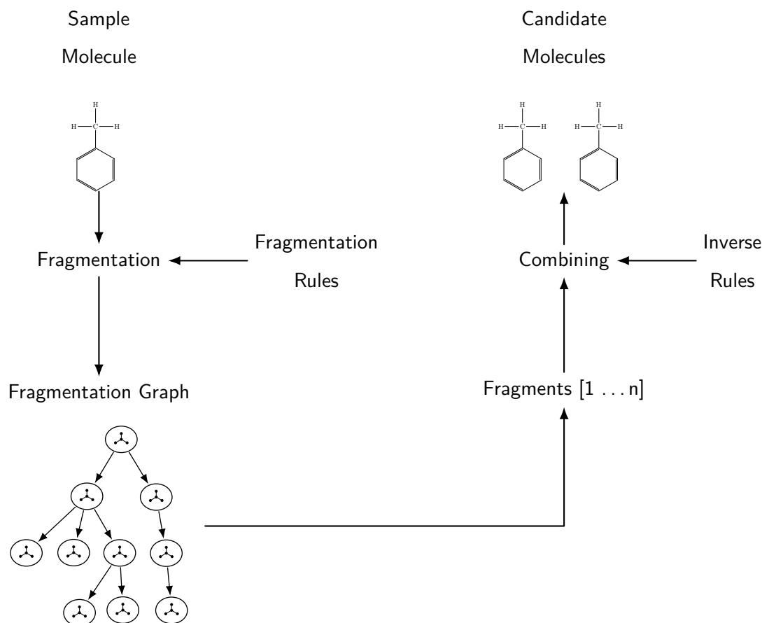
Figure 3.1: Schematic overview of the synthetic data-generation workflow. Starting from a sample molecule, fragmentation rules are applied to generate a fragmentation hypergraph that represents possible fragment formation pathways (left). The resulting fragments can also be recombined according to inverse rules to enumerate candidate molecules consistent with a given fragment set (right). Both directions are produced by the same rule-based graph-transformation pipeline, yielding the molecule–fragment data used to train the model.
