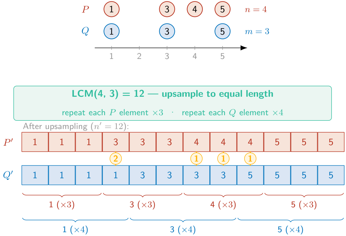
Figure 2.10: The inputs have different lengths, P = [1, 3, 4, 5] ( n = 4 ) and Q = [1, 3, 5] ( m = 3 ), so they are first brought to a common length before matched-pair differences can be formed. Each is upsampled to \text{LCM}(4, 3) = 12 by repeating every element of P three times and every element of Q four times (red and blue braces), giving aligned vectors P' = [1, 1, 1, 3, 3, 3, 4, 4, 4, 5, 5, 5] and Q' = [1, 1, 1, 1, 3, 3, 3, 3, 5, 5, 5, 5] . The amber badges mark the four index positions where the upsampled entries differ, with per-index gaps 2, 1, 1, 1. The Wasserstein distance is the mean of these absolute differences (see eq. (2.4)), showing how repetition lets each value contribute mass in proportion to its share of the original vector, so distributions of different cardinality can be compared directly.
