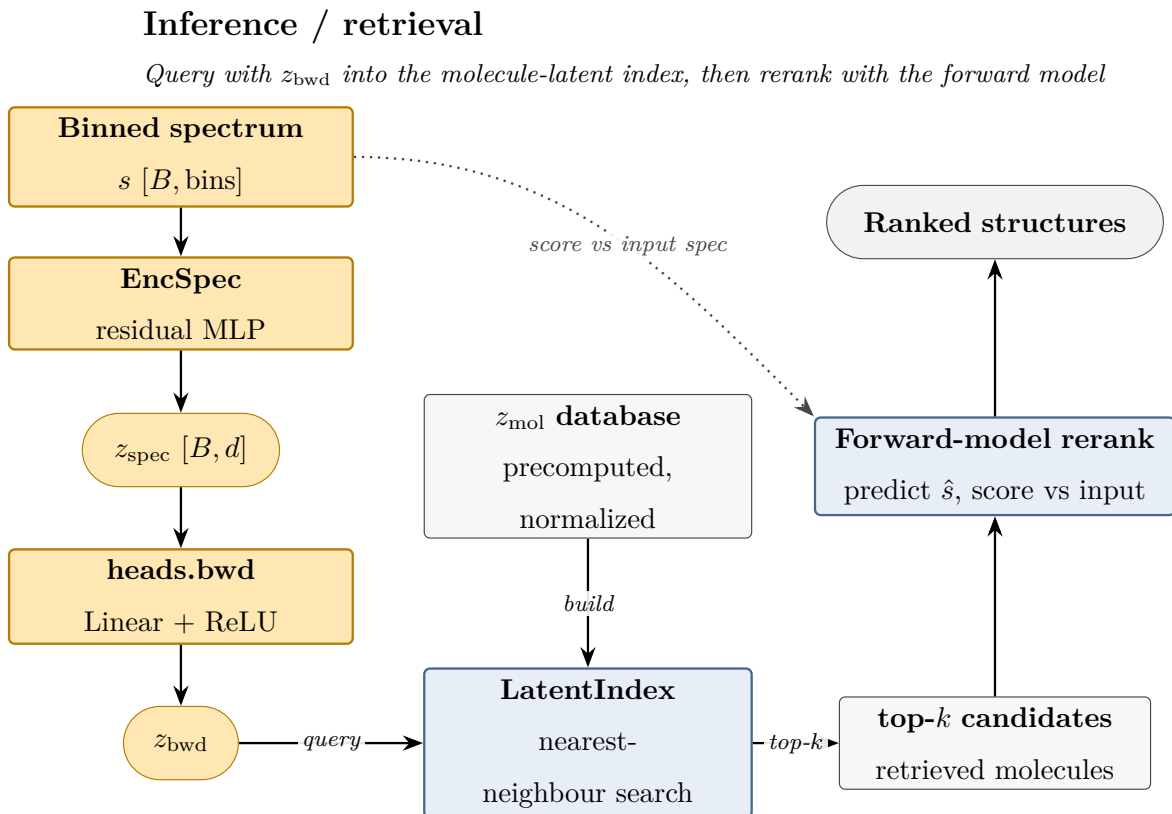
Figure 3.9: Inference-time spectrum-to-structure retrieval. A query spectrum is encoded to z_{\text{bwd}} through \text{Enc}_{\text{Spec}} and \text{Head}_{\text{BWD}} and used as a nearest-neighbour query against the molecular index—a precomputed store of normalized molecular latents z_{\text{mol}} ( build ). The retrieved top-k candidates are then reranked by the forward model, which predicts each candidate’s spectrum and scores it against the observed input, yielding the final ranked structures.
