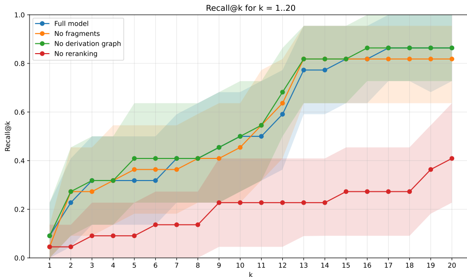
Figure 4.4: Recall@ k for k = 1, \dots, 20 across the full retrieval model and three ablated variants. Shaded bands show 95% bootstrap confidence intervals over queries. The full model and the no fragments / no derivation graph variants cluster together across the full k range, while the no reranking variant trails the others at every k , with the largest gap at small k and gradual closure toward k = 20 .
