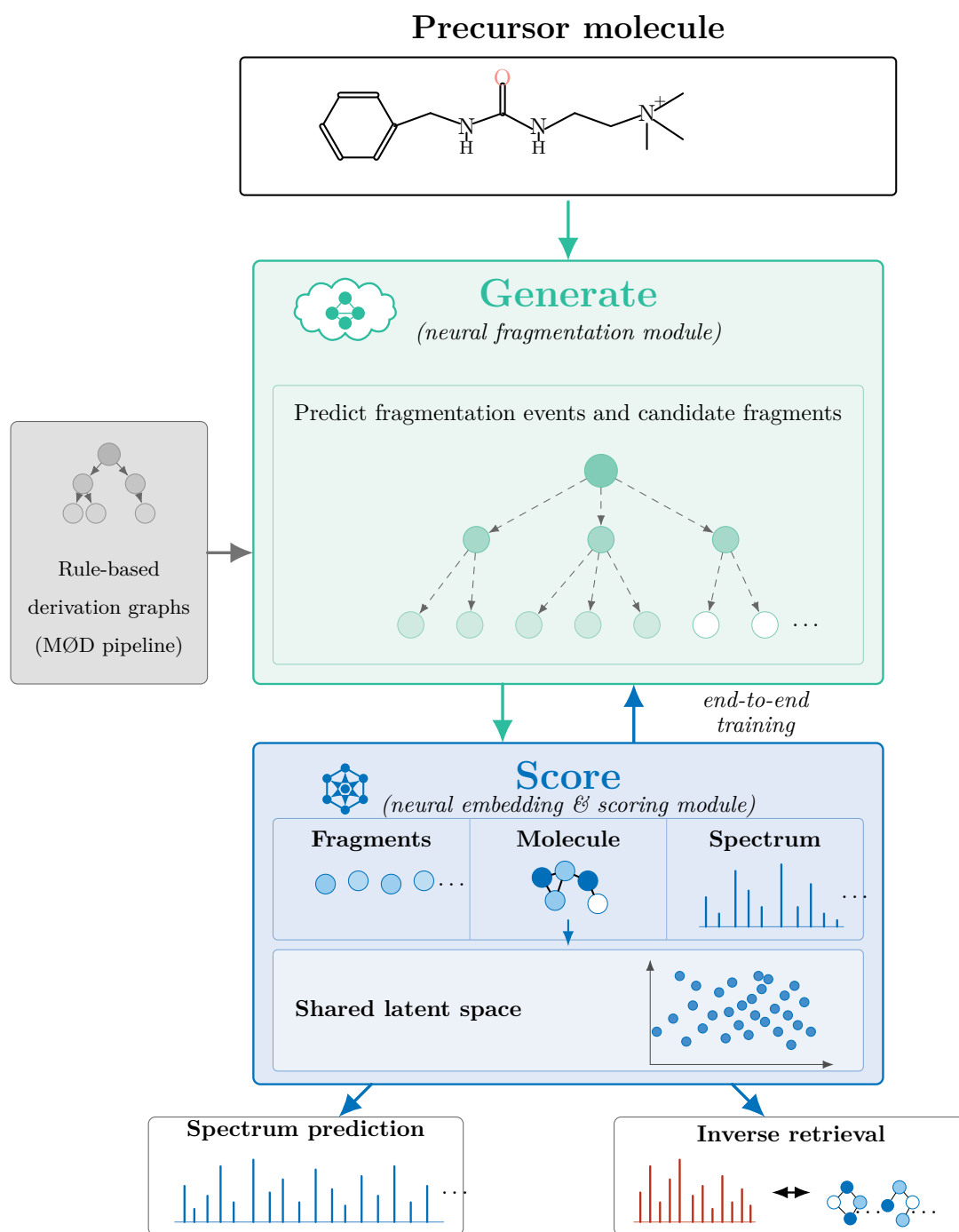
Figure 5.1: A future extension of the present work: shifting from fragment-structure encoding to fragmentation-process learning , so that the fragmentation graph becomes a predicted object rather than a fixed input.
