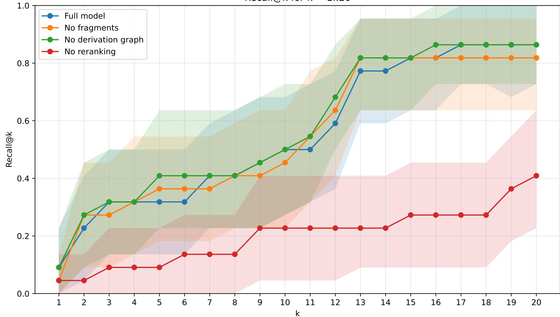
Recall@k for k = 1..20
