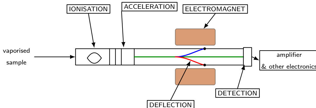
Figure 2.2: Simplified schematic of the measurement principle in a magnetic sector mass spectrometer. Following sample introduction, ionisation and acceleration generate an ion beam that is separated in the magnetic field by deflection that depends on m/z . The separated ions are then detected and transformed into an electrical signal for further processing. [20]
