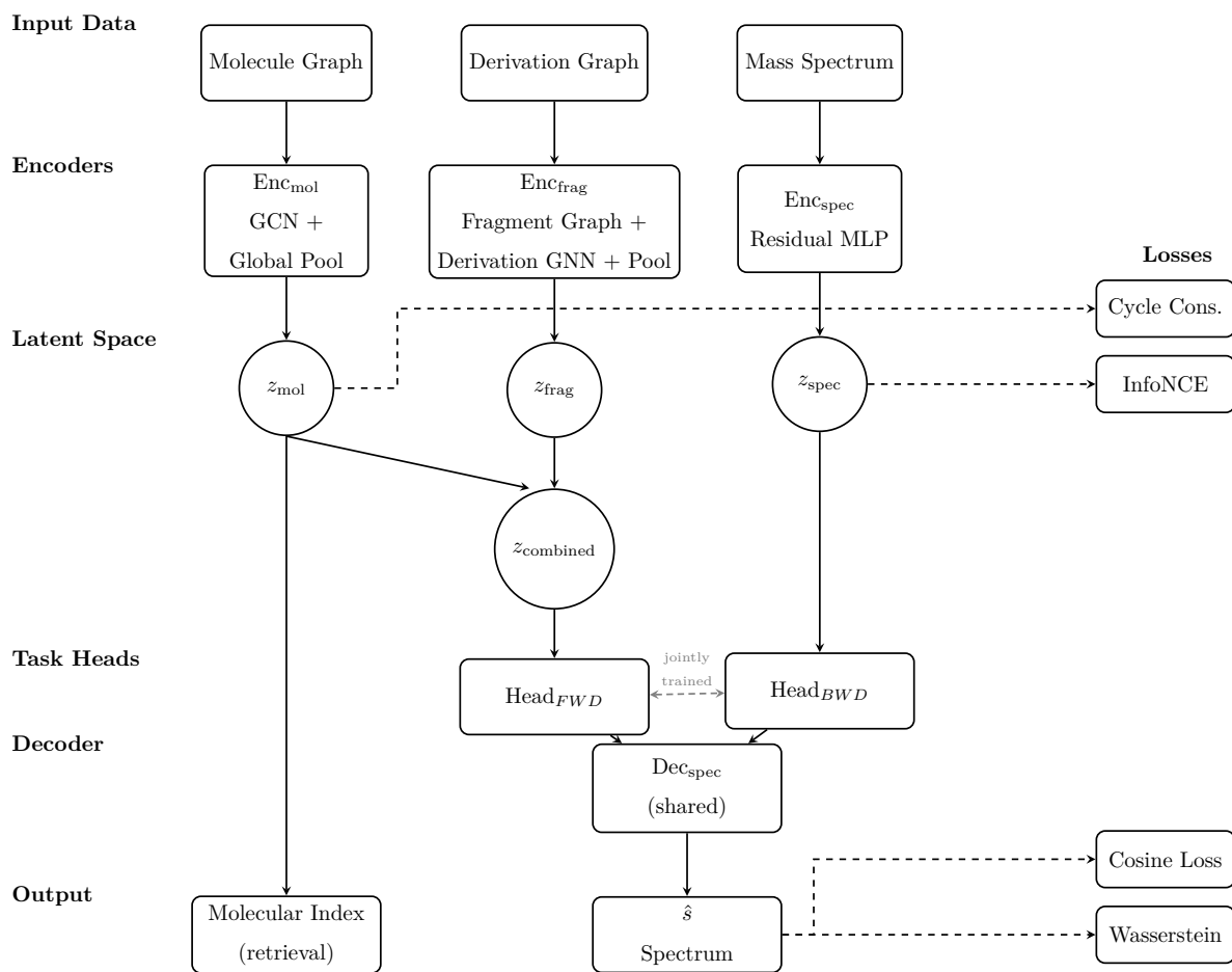
Figure 3.8: Diagram illustrating the overall architecture of the bidirectional translation framework, showing the flow from molecular graph encoding to spectral embedding and back.
