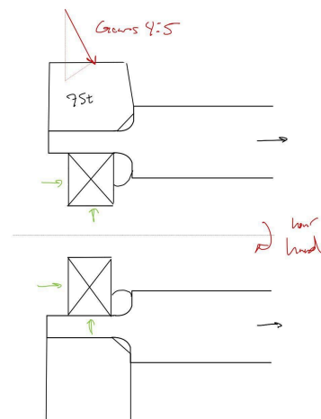
Figure 5. Primary Shaft, Sleeve FBD
