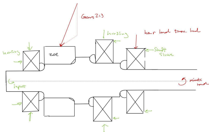
Figure 3. Intermediate Shaft FBD
