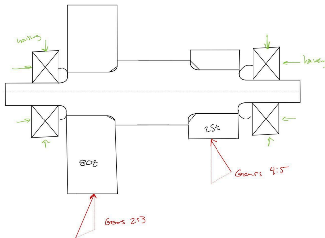
Figure 3. Intermediate Shaft FBD
