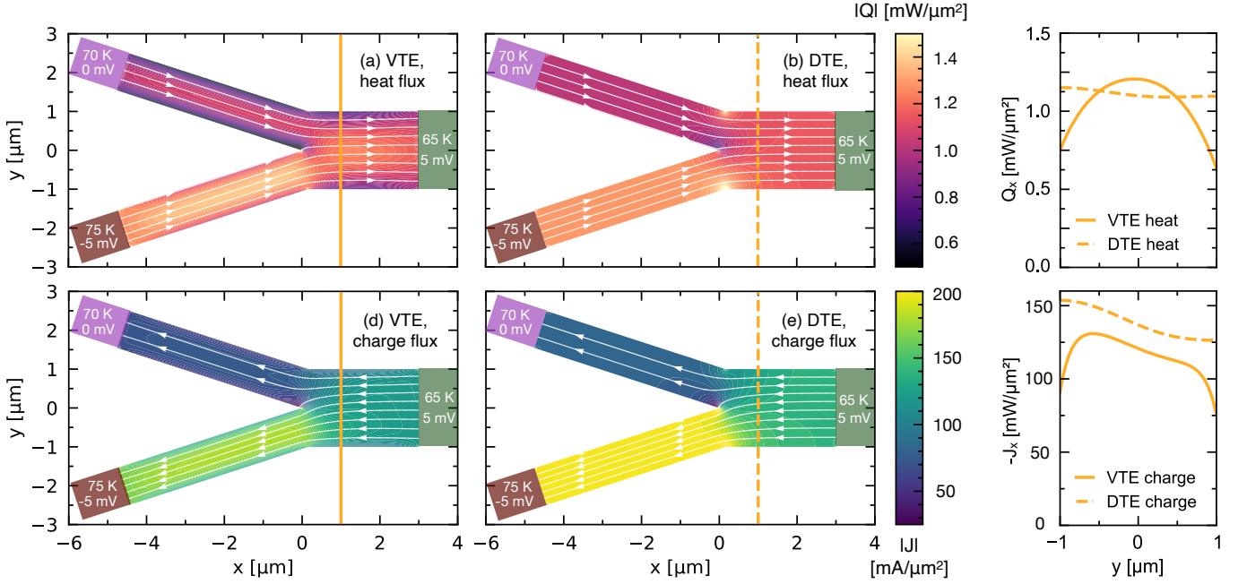
FIG. 2. Macroscopic signatures of viscous electron-phonon hydrodynamics , along the in-plane direction of a fluid-mixing device made of graphite. Boundary conditions are as follows: temperature (potential) is set at 70 K (0 mV) on the upper thin terminal, 75 K (−5 mV) on the lower thin terminal, and at 65 K (5 mV) at the wide terminal. A zero total heat and charge flux is imposed at the other boundaries, in the VTE case, electron and phonon drift velocities are zero on all boundaries (no-slip BCs). Top row, heat flux predicted from the VTE (a), or DTE (b) and their comparison along the section x=1\mu\text{m} (c). Bottom row, charge flux predicted from the VTE (d), DTE (e), and their comparison along the section x=1\mu\text{m} (f).
