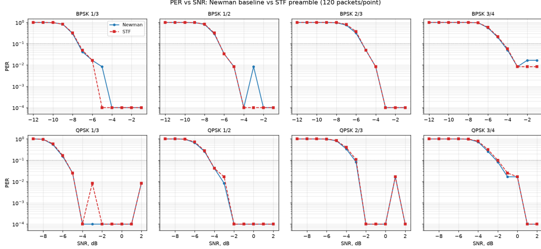
Figure 5: PER versus SNR for the Newman-tone and STF preamble variants over the article channel (same channel realizations per arm).
