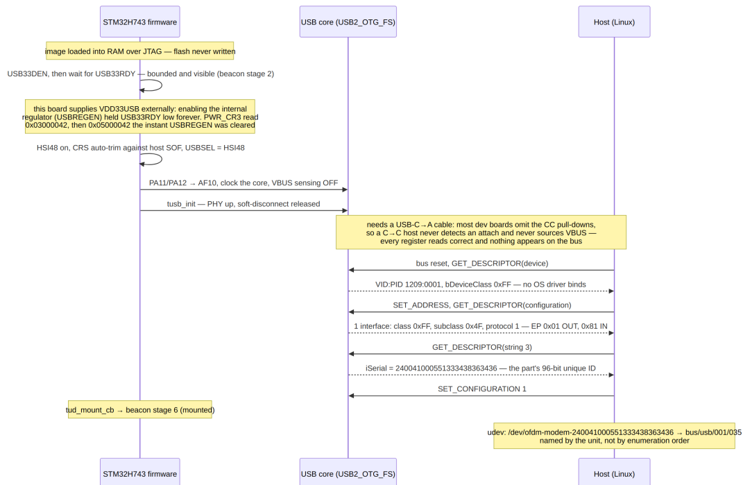
Figure 41: Enumeration: supply detection, clocks from HSI48 (trimmed against the host’s SOF, so the firmware is correct whatever the board’s crystal), and the descriptors that give the device its identity.
