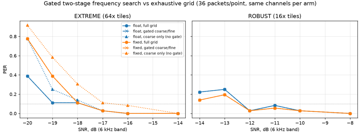
Figure 25: PER versus SNR for the exhaustive frequency grid (solid), the gated two-stage search (dashed), and the ungated coarse-only ablation (dotted); float and fixed-point receivers, same channels per arm. Gated overlays full exactly everywhere; the ablation’s edge loss in the EXTREME panel is what the contrast gate prevents.
