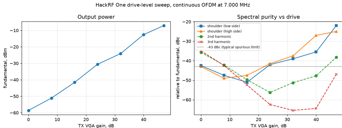
Figure 33: Drive-level sweep on the HackRF One ( demoapp/sdr_drive_sweep.py ): output power, and spectral purity relative to the fundamental, against transmit gain. Points below VGA 16 are limited by the analyser’s noise floor, not by the transmitter.
