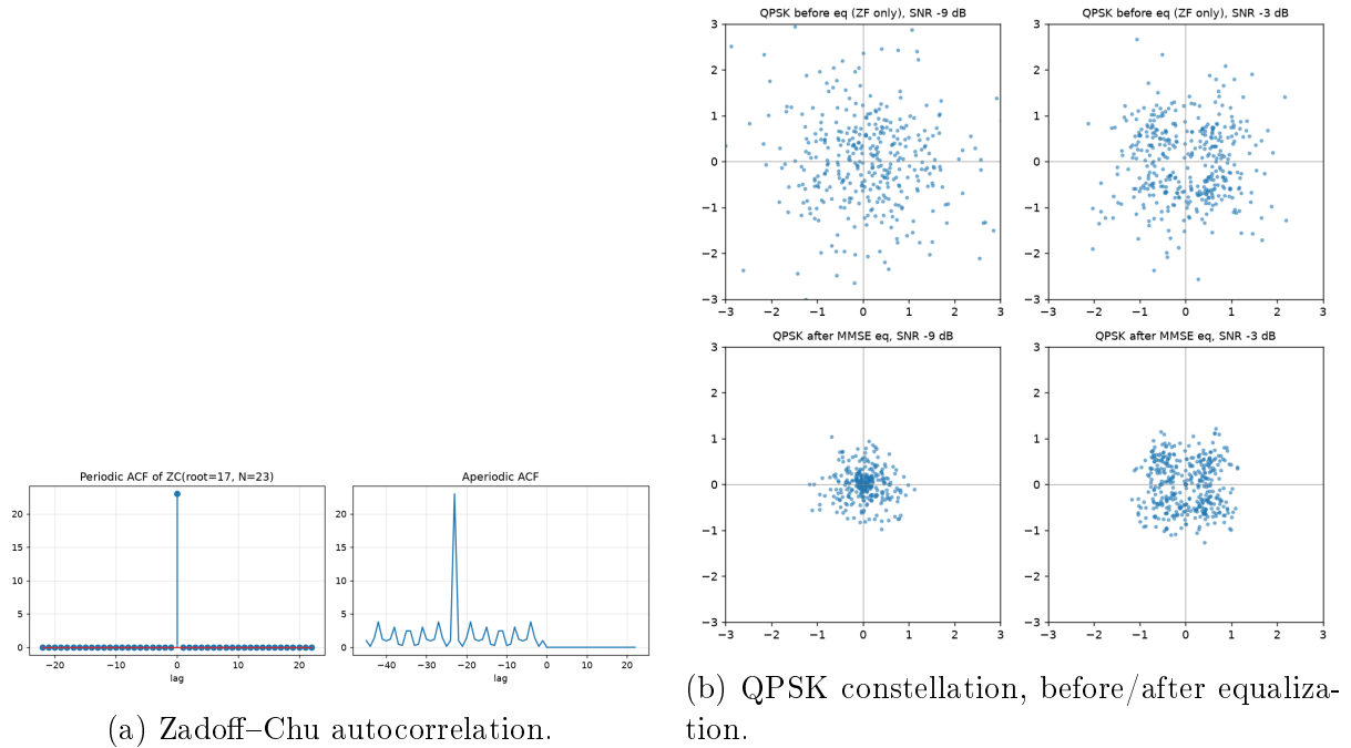
Figure 27: Article-style diagnostic figures ( experiments/figures.py ).
