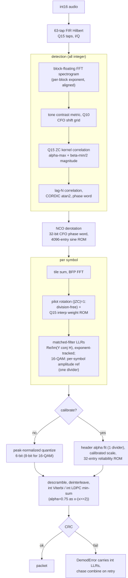
Figure 24: Fixed-point receiver datapath (all integer).
