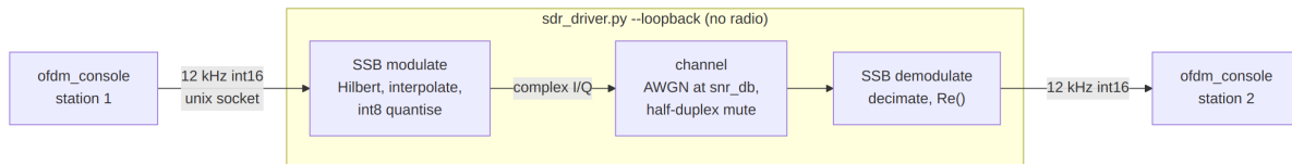
Figure 30: Hardware-free loopback: two stations cross-connected through the full SSB modulation and demodulation chain.
