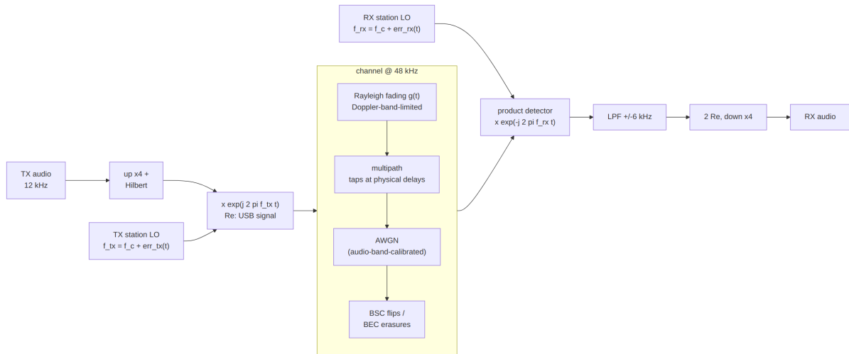
Figure 22: The RF chain: USB modulator, 48 kHz channel (fading, multipath, AWGN, BSC/BEC), product detector.
