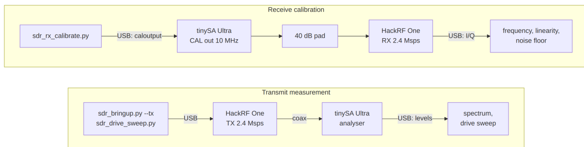
Figure 31: Instrumented bench, both directions: as an analyser the tinySA measures what the radio transmits; as a source its calibration output drives the receiver through a 40 dB pad.
