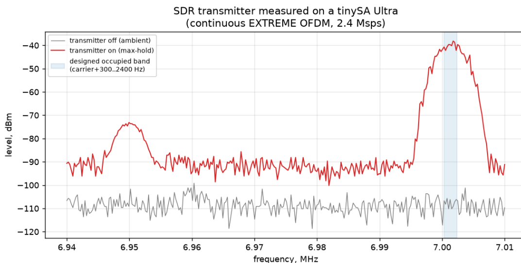
Figure 32: The transmitter measured on a tinySA Ultra: continuous EXTREME OFDM at 2.4 Msps, carrier 7.000 MHz, 3 kHz RBW. The shaded band is the designed occupancy (carrier + 300...2400 Hz); the spur at 6.95 MHz is the offset-tuned local oscillator.
