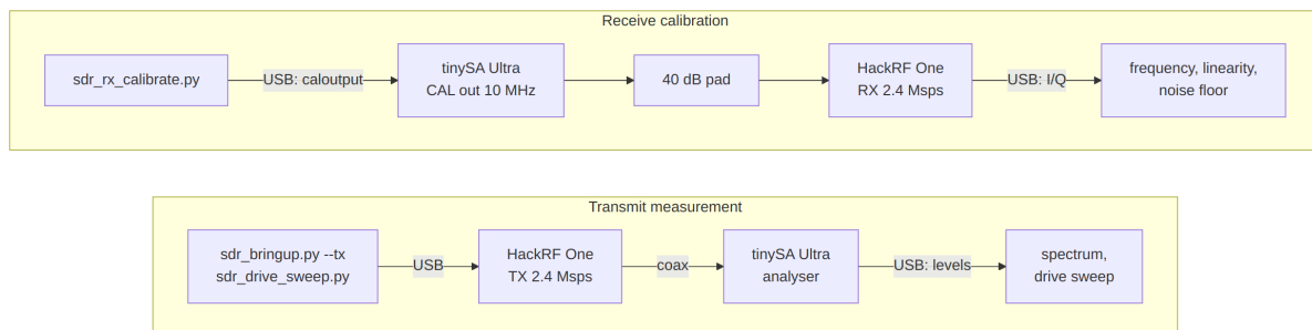
Figure 49: Instrumented bench, both directions: as an analyser the tinySA measures what the radio transmits; as a source its calibration output drives the receiver through a 40 dB pad.
