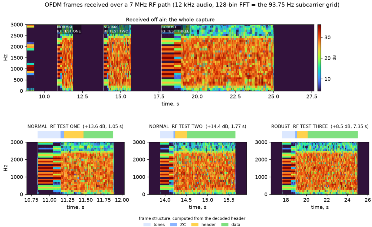
Figure 54: Frames received over the air ( demoapp/sdr_waterfall.py on results/am_rx_offair.wav ): the whole capture above, each frame below with its measured structure. The ROBUST frame carries the same 27 bytes as its NORMAL neighbours and occupies 7.35 s doing it — what 16\times tiling costs, and buys.
