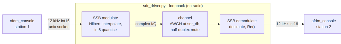
Figure 48: Hardware-free loopback: two stations cross-connected through the full SSB modulation and demodulation chain.
