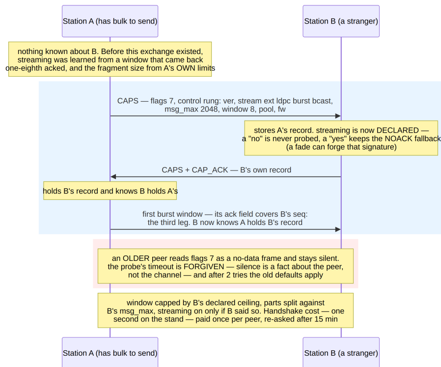
Figure 46: The three-leg capability handshake. The record rides the third impossible flag combination, so an older peer reads it as a no-data frame and simply does not answer — which is itself the answer, and is forgiven rather than charged to the rate controller.
