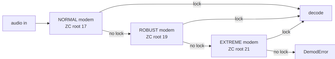
Figure 9: Blind mode detection: the preamble root is the mode signal. A consequence used throughout the link layer: a mode switch can never deadlock the link.
