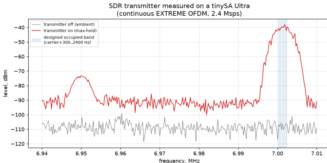
Figure 47: The transmitter measured on a tinySA Ultra: continuous EXTREME OFDM at 2.4 Msps, carrier 7.000 MHz, 3 kHz RBW. The shaded band is the designed occupancy (carrier + 300...2400 Hz); the spur at 6.95 MHz is the offset-tuned local oscillator.
