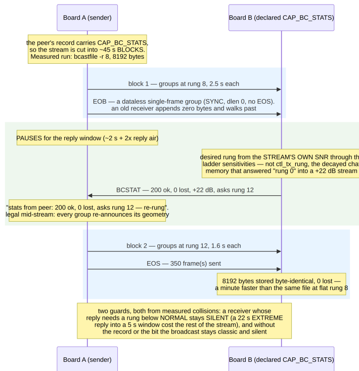
Figure 31: Block statistics and the mid-stream re-rung, with the measured run’s numbers. Both guard rules at the bottom came from collisions the first live runs produced.
