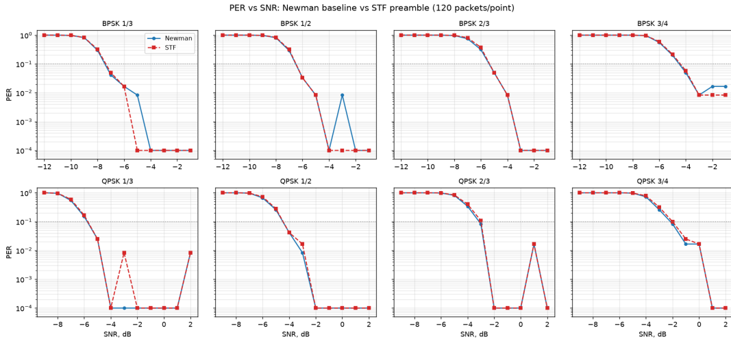
Figure 8: PER versus SNR for the Newman-tone and STF preamble variants over the article channel (same channel realizations per arm).
