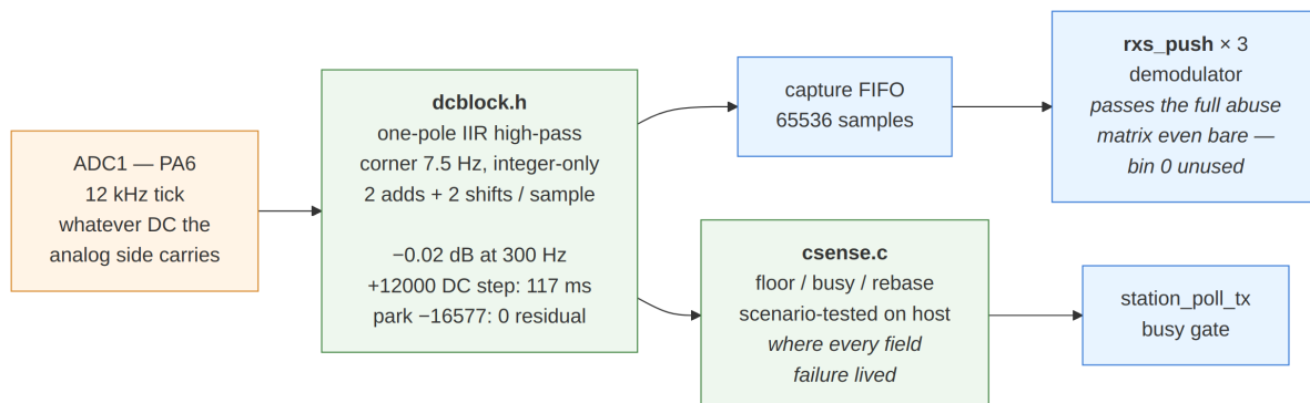
Figure 36: The DC-blind front end. One integer high-pass at the input makes every consumer indifferent to the analog operating point; carrier sense — where every field failure of the campaign lived — is a shared module with a host scenario suite.
