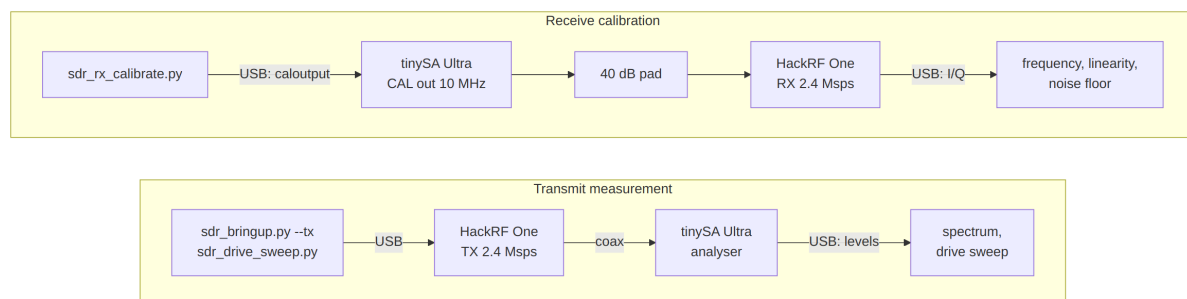
Figure 46: Instrumented bench, both directions: as an analyser the tinySA measures what the radio transmits; as a source its calibration output drives the receiver through a 40 dB pad.
