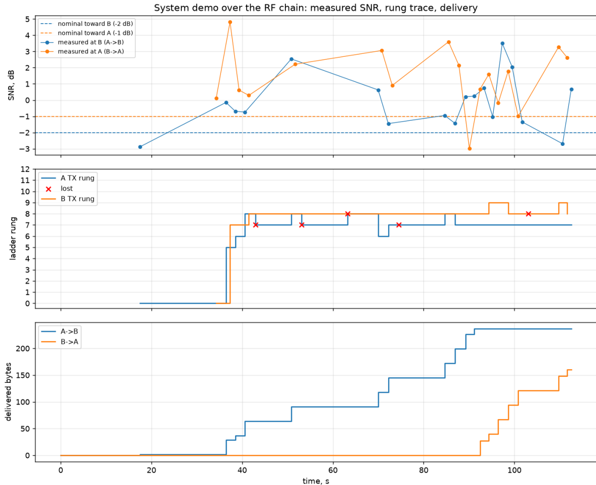
Figure 56: System-demo timeline: per-frame SNR, ladder rungs, and delivery over the session.
