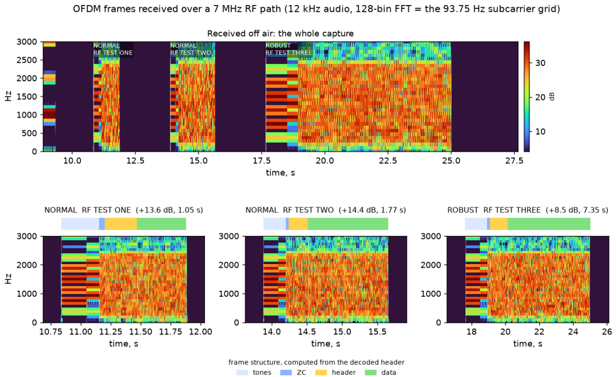
Figure 50: Frames received over the air (demoapp/sdr_waterfall.py on results/am_rx_offair.wav): the whole capture above, each frame below with its measured structure. The ROBUST frame carries the same 27 bytes as its NORMAL neighbours and occupies 7.35 s doing it — what 16× tiling costs, and buys.
