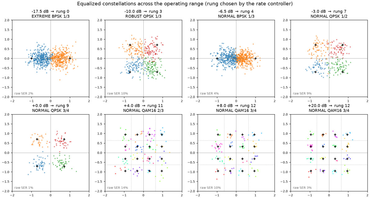
Figure 10: Equalized constellations at the controller-selected rung, from the EXTREME sensitivity floor to a clean channel (article channel, AWGN + CFO). Black crosses mark the ideal constellation points; each received point is colored by the transmitted symbol, so raw pre-FEC errors appear as points of the wrong color inside a neighbouring decision region (the per-panel “raw SER” annotation counts them), and the dotted subgrid on the 16-QAM panels marks the decision boundaries between the 16 cells.
