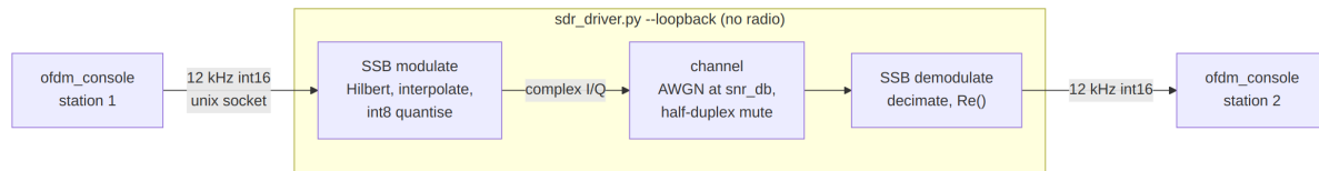
Figure 45: Hardware-free loopback: two stations cross-connected through the full SSB modulation and demodulation chain.
