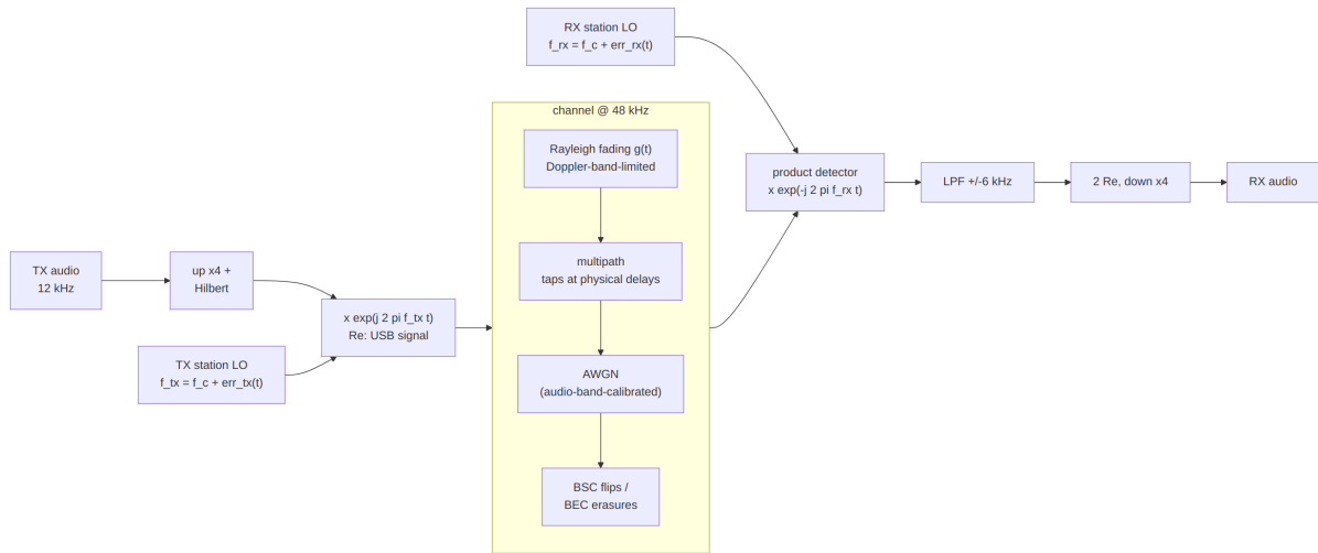
Figure 2: The RF chain: USB modulator, 48 kHz channel (fading, multipath, AWGN, BSC/BEC), product detector.
