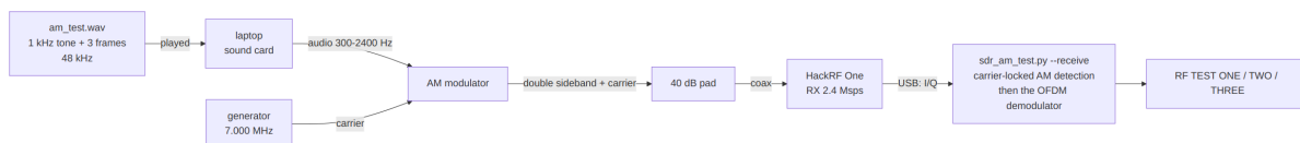
Figure 49: Off-air receive test: an external AM transmitter feeds the SDR through a 40 dB pad.
