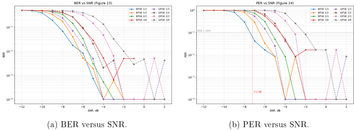
Figure 54: Reproduction of the article’s Figures 23–24: eight modulation/rate configurations over the article channel model (multipath [1, 0, 0.4, 0, 0, 0.2] , BSC 10^{-3} , BEC 2 \cdot 10^{-2} , random \pm 100 Hz CFO with drift, random timing), 120 packets per point.
