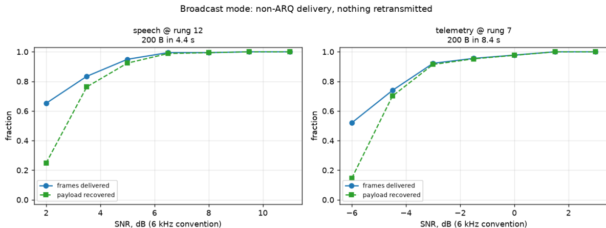
Figure 26: Non-ARQ delivery against SNR. Frames delivered runs above payload recovered at the low end because a frame lost from the middle of a group costs its own bytes while still being counted in the span.
