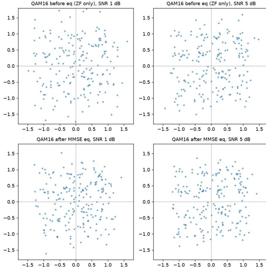
Figure 18: 16-QAM received constellations over the article channel ( experiments/figures.py ): before equalization (ZF pilot estimate only, top) and after Wiener-refined MMSE equalization (bottom), at the bottom (+1 dB) and top (+5 dB) of the 16-QAM operating range.
