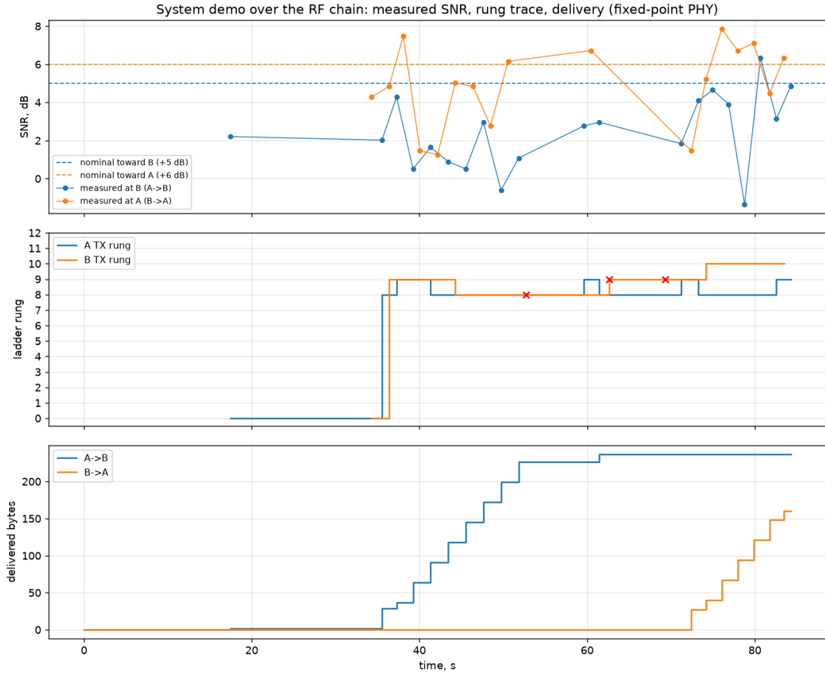
Figure 57: Fixed-point-pipeline demo at +5dB: the integer SNR estimates drive the ladder into the 16-QAM rungs.
