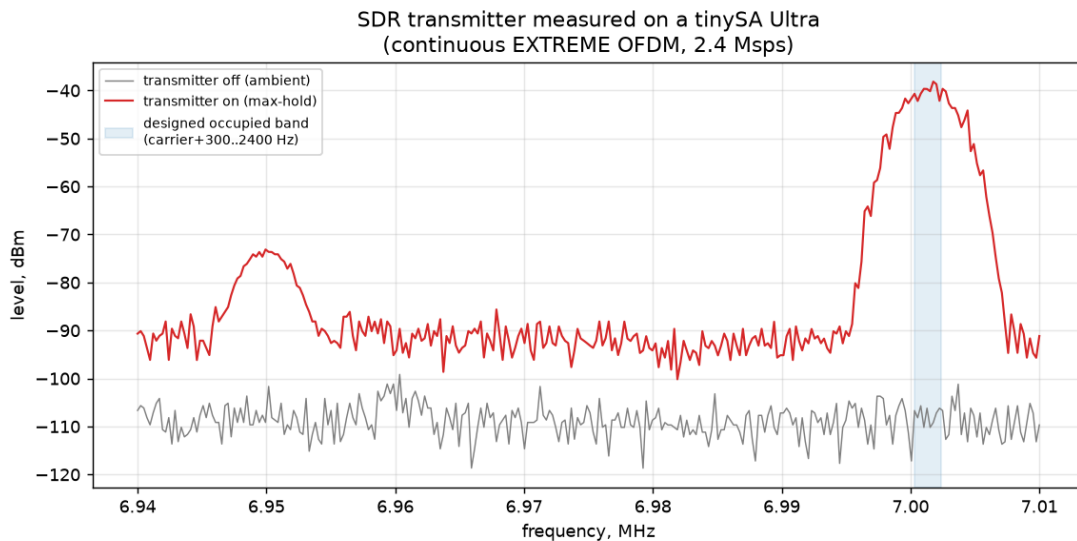
Figure 47: The transmitter measured on a tinySA Ultra: continuous EXTREME OFDM at 2.4 Mps, carrier 7.000 MHz, 3 kHz RBW. The shaded band is the designed occupancy (carrier + 300...2400 Hz); the spur at 6.95 MHz is the offset-tuned local oscillator.
