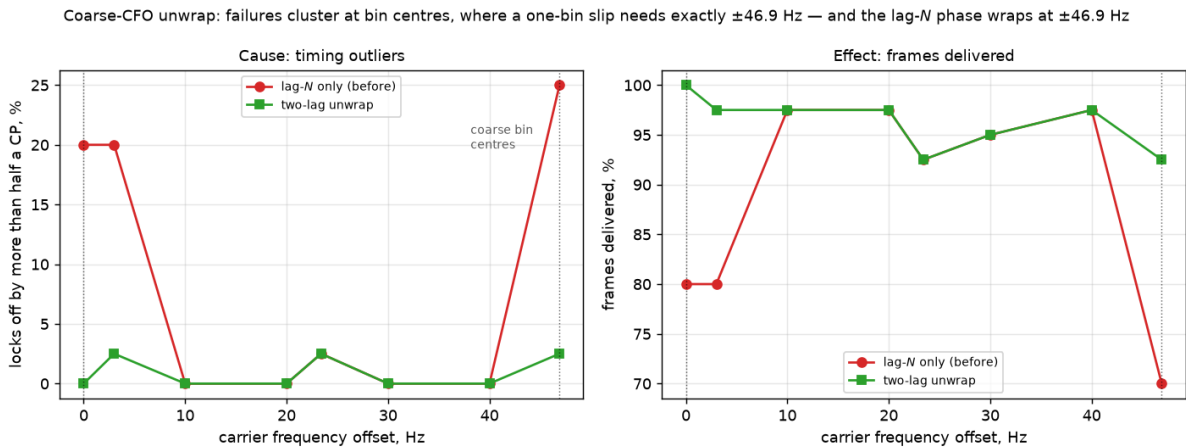
Figure 29: The coarse-CFO unwrap swept across one bin ( experiments/cfo_unwrap.py , QPSK 1/2 at -3.5 dB, 40 frames per point). Dotted lines mark the coarse bin centres.
