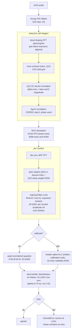
Figure 27: Fixed-point receiver datapath (all integer).
