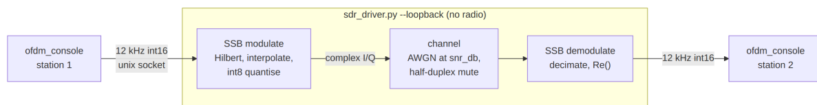
Figure 35: Hardware-free loopback: two stations cross-connected through the full SSB modulation and demodulation chain.
