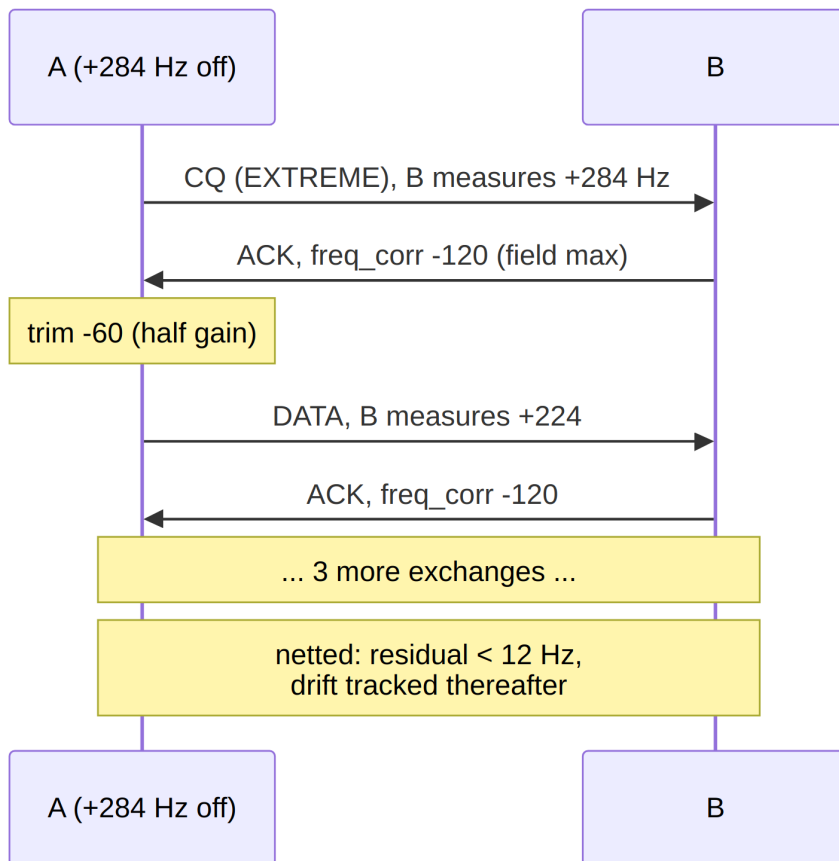
Figure 24: AFC netting from a +284 Hz initial offset.
