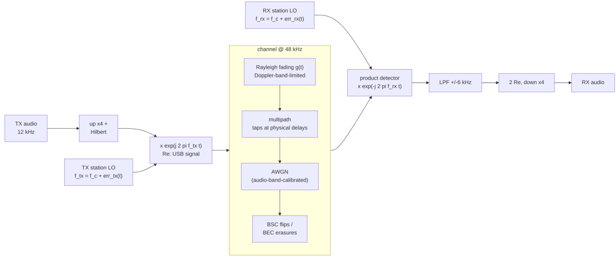
Figure 25: The RF chain: USB modulator, 48 kHz channel (fading, multipath, AWGN, BSC/BEC), product detector.
