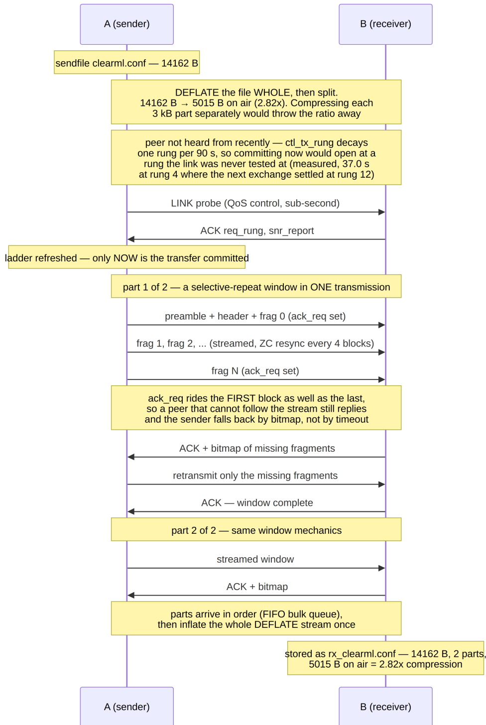
Figure 34: A file transfer: whole-file compression, a link probe before the transfer is committed, then selective-repeat windows carried one per transmission.
