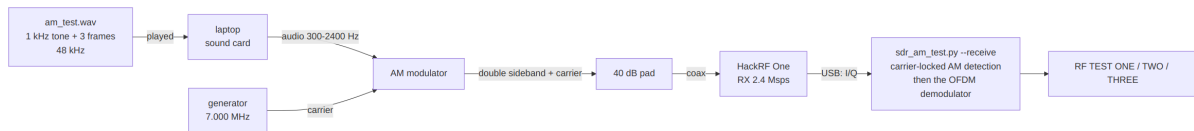
Figure 39: Off-air receive test: an external AM transmitter feeds the SDR through a 40 dB pad.
