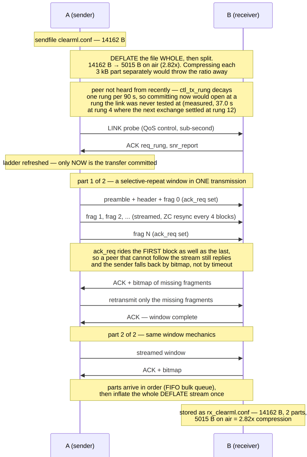
Figure 39: A file transfer: whole-file compression, a link probe before the transfer is committed, then selective-repeat windows carried one per transmission.
