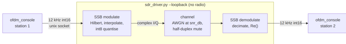
Figure 40: Hardware-free loopback: two stations cross-connected through the full SSB modulation and demodulation chain.
