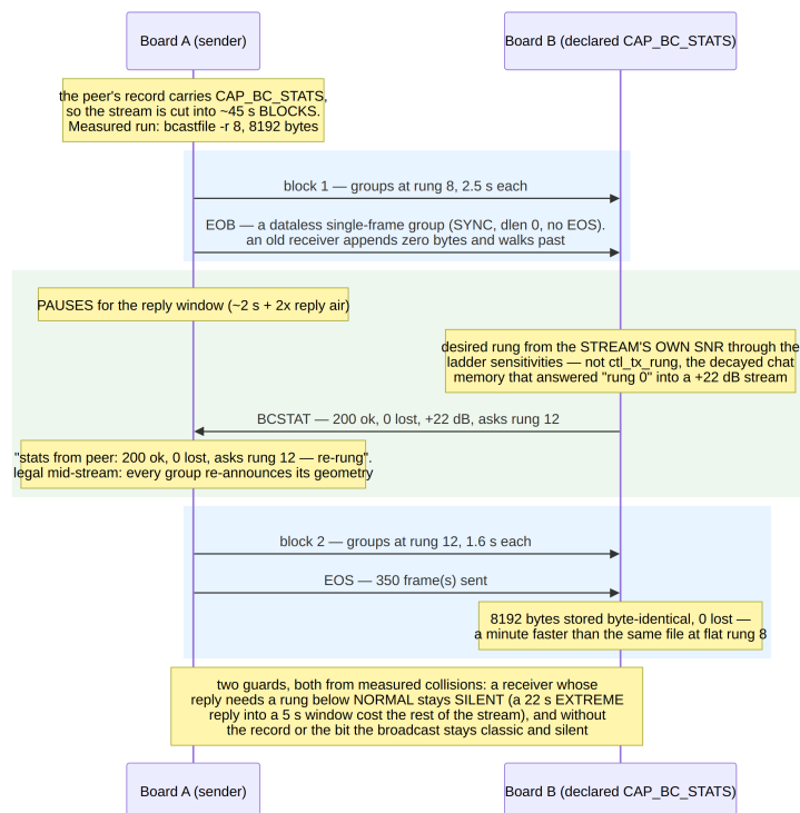
Figure 45: Block statistics and the mid-stream re-rung, with the measured run's numbers. Both guard rules at the bottom came from collisions the first live runs produced.
