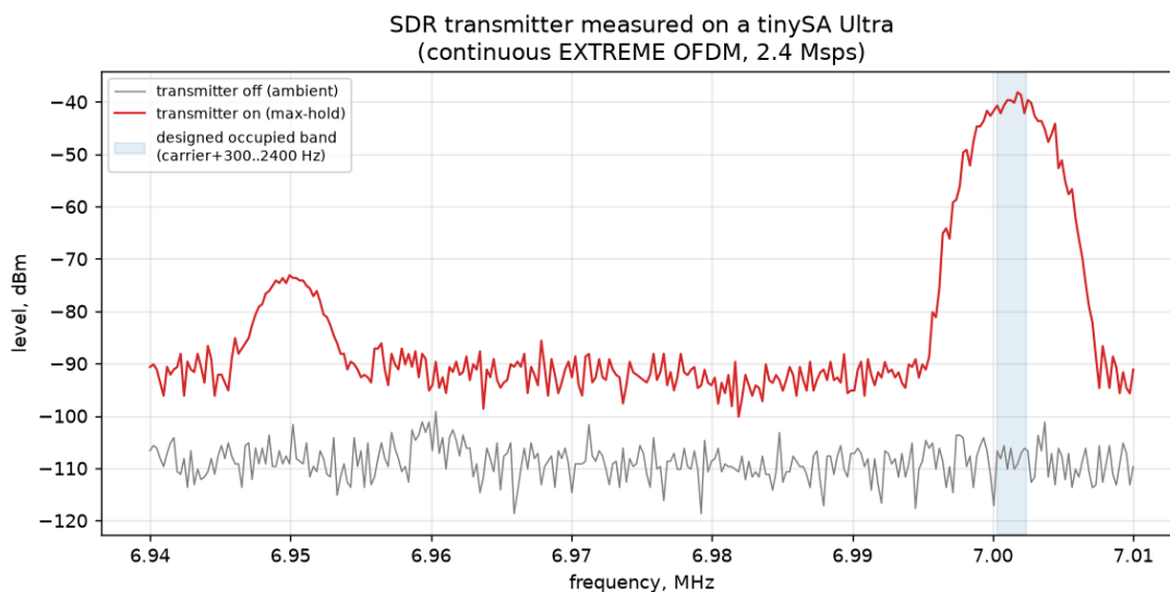
Figure 51: The transmitter measured on a tinySA Ultra: continuous EXTREME OFDM at 2.4 Msps, carrier 7.000 MHz, 3 kHz RBW. The shaded band is the designed occupancy (carrier + 300...2400 Hz); the spur at 6.95 MHz is the offset-tuned local oscillator.
