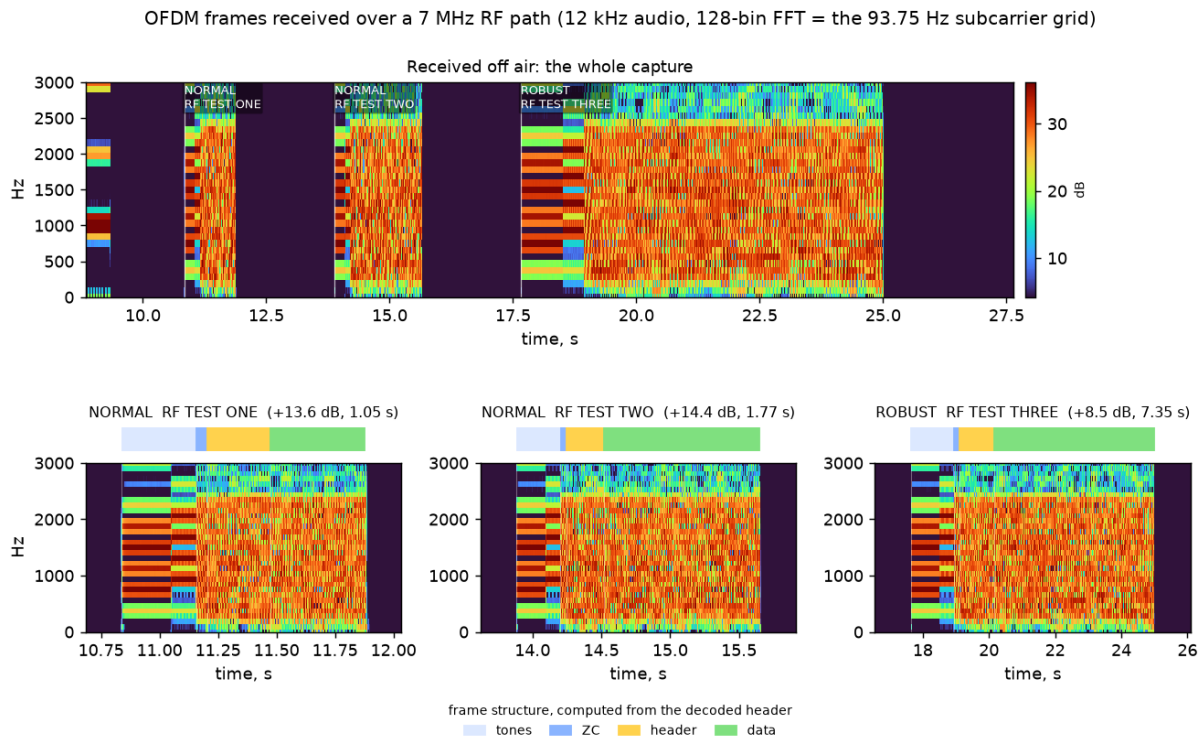
Figure 37: Frames received over the air ( demoapp/sdr_waterfall.py on results/am_rx_offair.wav ): the whole capture above, each frame below with its measured structure. The ROBUST frame carries the same 27 bytes as its NORMAL neighbours and occupies 7.35 s doing it — what 16\times tiling costs, and buys.
