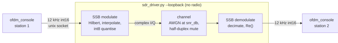
Figure 31: Hardware-free loopback: two stations cross-connected through the full SSB modulation and demodulation chain.
