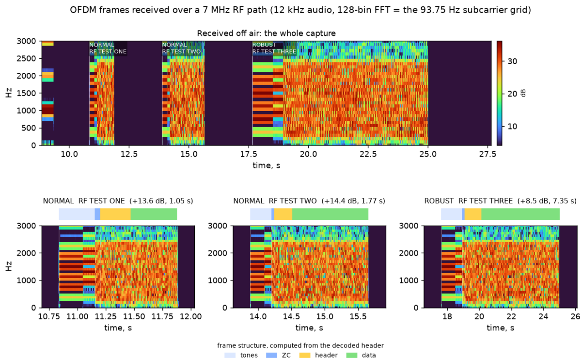
Figure 36: Frames received over the air (demoapp/sdr_waterfall.py on results/am_rx_offair.wav): the whole capture above, each frame close up below with its preamble, header and data spans marked.
