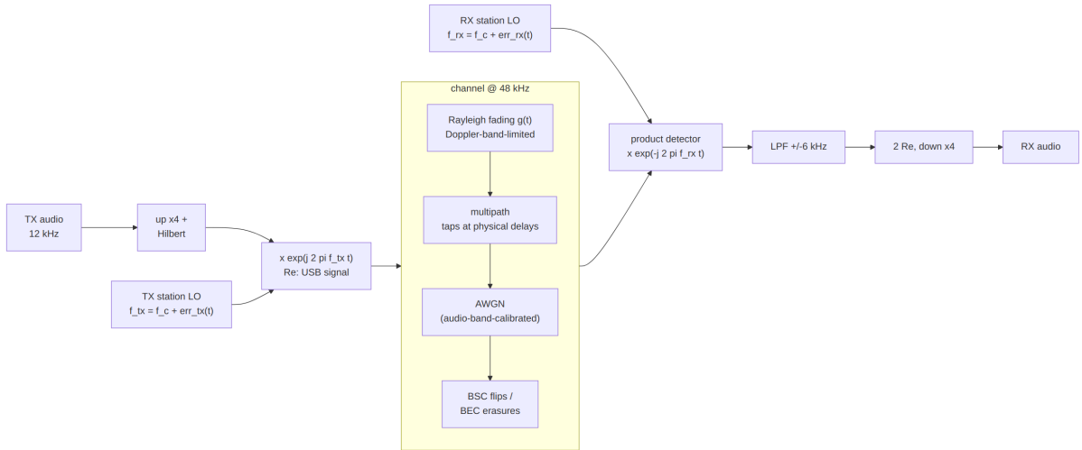
Figure 23: The RF chain: USB modulator, 48 kHz channel (fading, multipath, AWGN, BSC/BEC), product detector.
