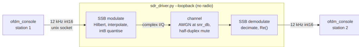
Figure 45: Hardware-free loopback: two stations cross-connected through the full SSB modulation and demodulation chain.
