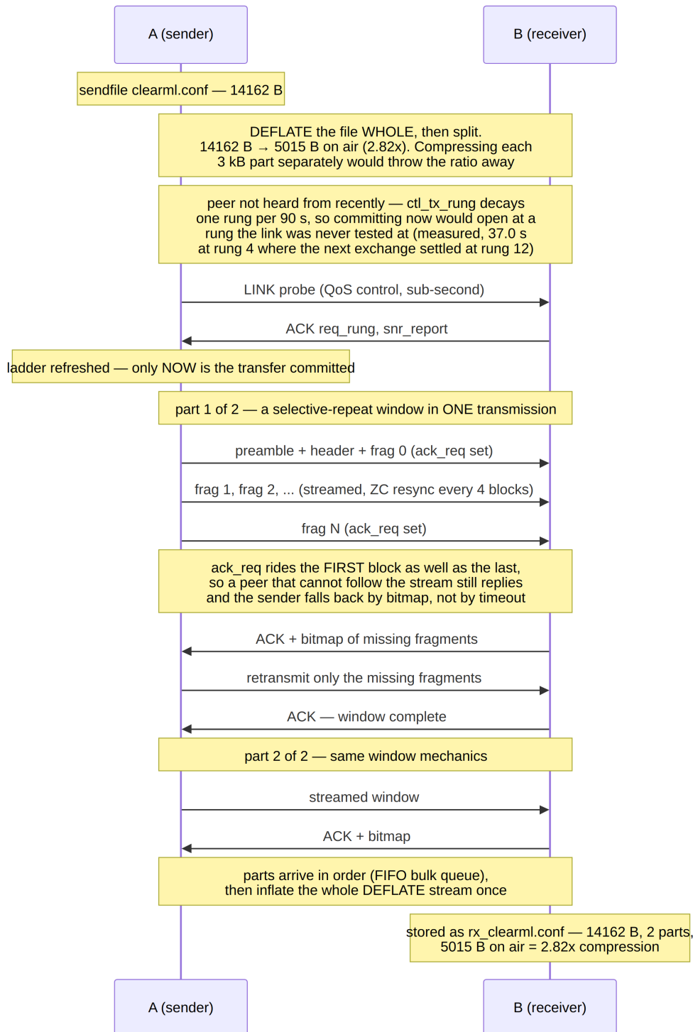
Figure 40: A file transfer: whole-file compression, a link probe before the transfer is committed, then selective-repeat windows carried one per transmission.
