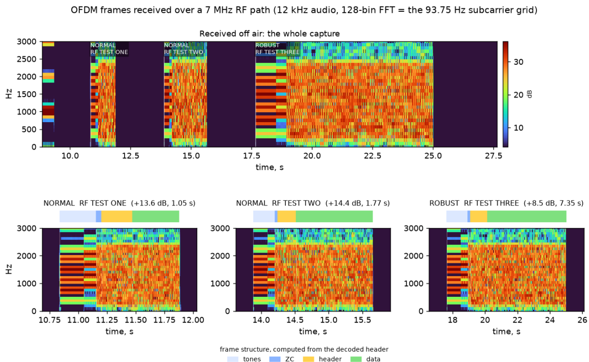
Figure 46: Frames received over the air (demoapp/sdr_waterfall.py on results/am_rx_offair.wav): the whole capture above, each frame close up below with its preamble, header and data spans marked.
