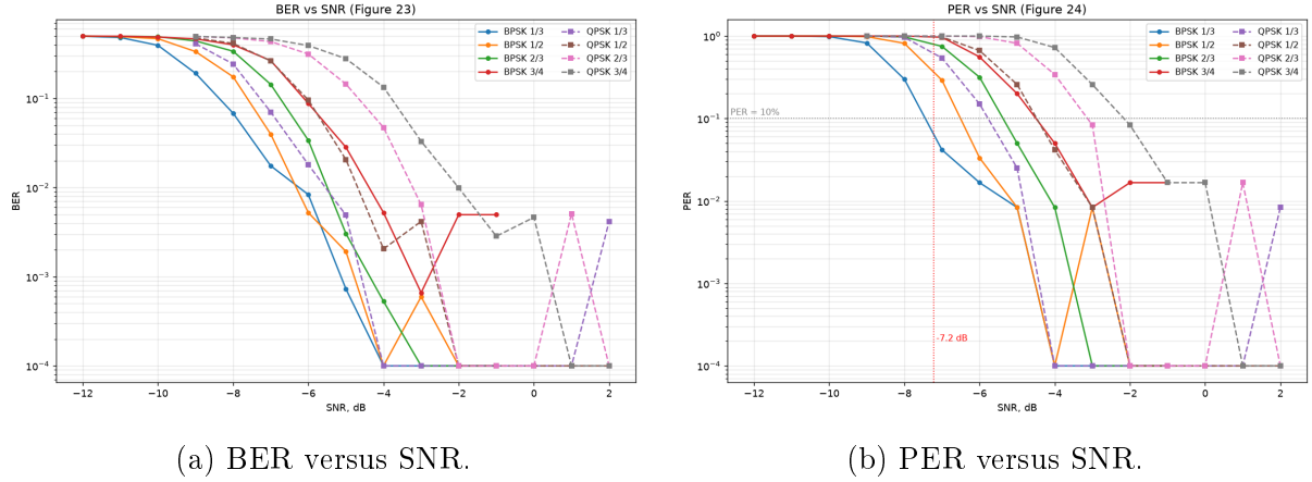
Figure 25: Reproduction of the article’s Figures 23–24: eight modulation/rate configurations over the article channel model (multipath [1, 0, 0.4, 0, 0, 0.2] , BSC 10^{-3} , BEC 2 \cdot 10^{-2} , random \pm 100 Hz CFO with drift, random timing), 120 packets per point.
