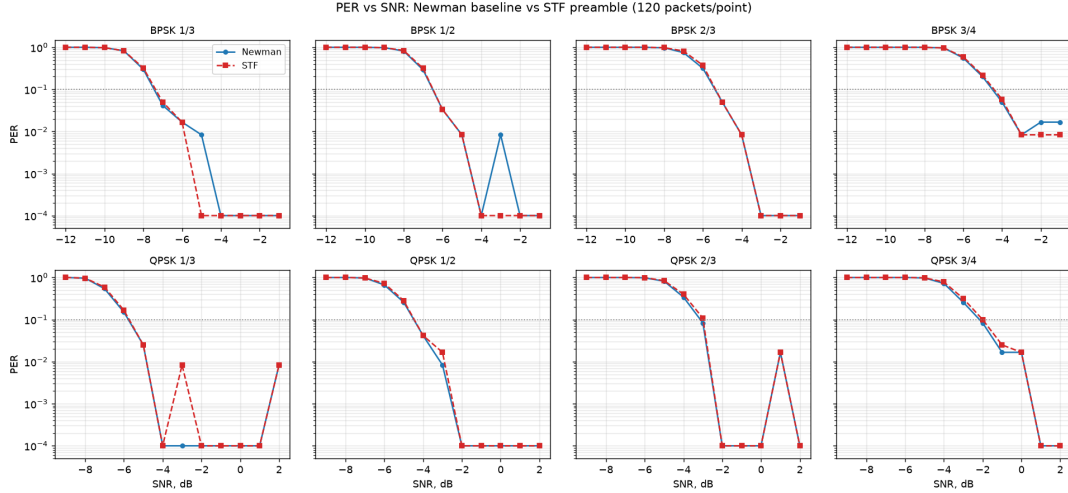
Figure 5: PER versus SNR for the Newman-tone and STF preamble variants over the article channel (same channel realizations per arm).
