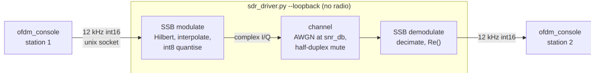
Figure 29: Hardware-free loopback: two stations cross-connected through the full SSB modulation and demodulation chain.
