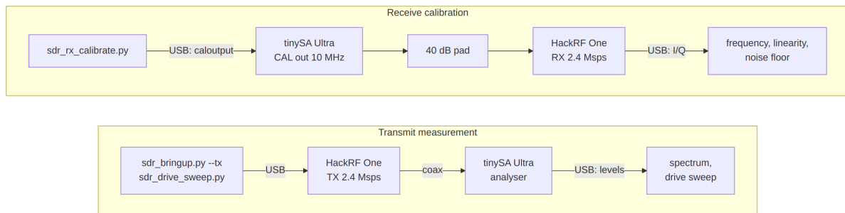
Figure 30: Instrumented bench, both directions: as an analyser the tinySA measures what the radio transmits; as a source its calibration output drives the receiver through a 40 dB pad.
