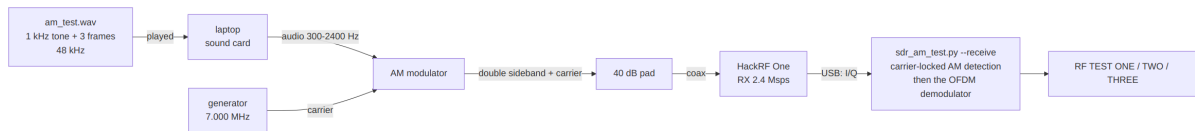
Figure 33: Off-air receive test: an external AM transmitter feeds the SDR through a 40 dB pad.
