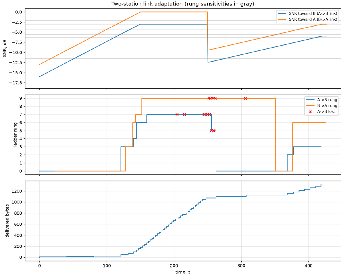
Figure 19: Controller-level two-station simulation ( experiments/link_adaptation.py ): asymmetric channel, -16 dB start, sudden fade; 1290/1500 bytes delivered at 24 bit/s effective goodput including ACK overhead and turnarounds.
