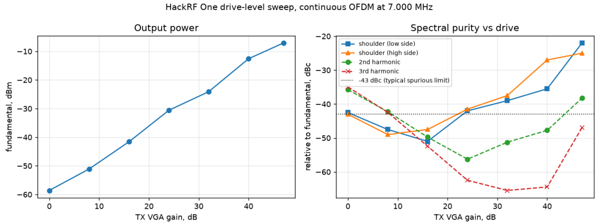
Figure 32: Drive-level sweep on the HackRF One ( demoapp/sdr_drive_sweep.py ): output power, and spectral purity relative to the fundamental, against transmit gain. Points below VGA 16 are limited by the analyser’s noise floor, not by the transmitter.
