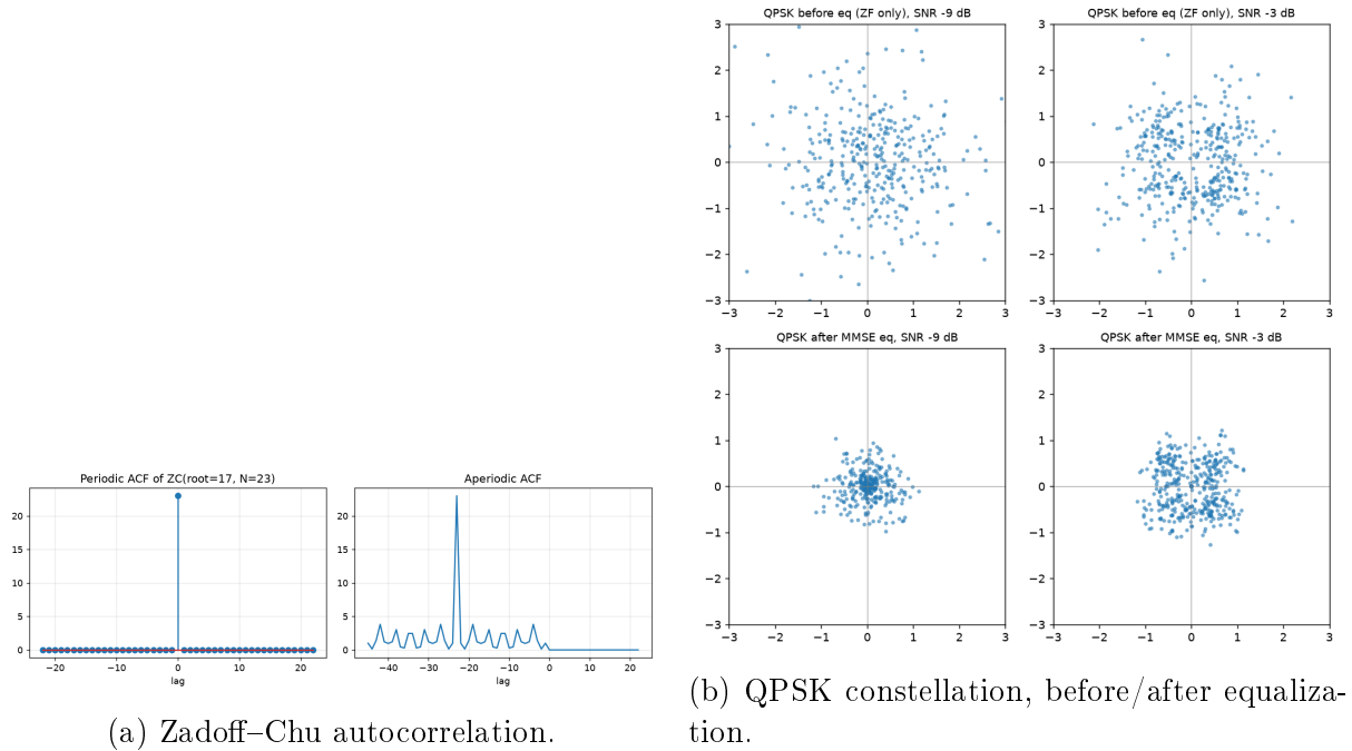
Figure 26: Article-style diagnostic figures ( experiments/figures.py ).
