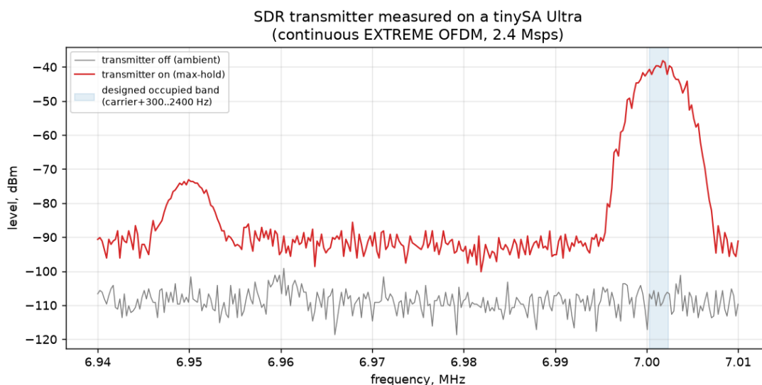
Figure 29: The transmitter measured on a tinySA Ultra: continuous EXTREME OFDM at 2.4 Msps, carrier 7.000 MHz, 3 kHz RBW. The shaded band is the designed occupancy (carrier + 300...2400 Hz); the spur at 6.95 MHz is the offset-tuned local oscillator.
