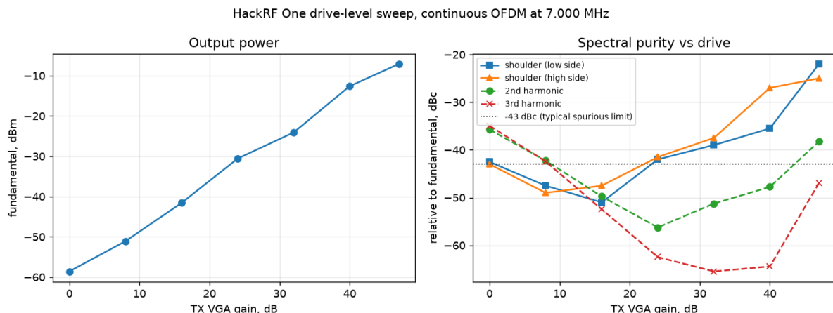
Figure 30: Drive-level sweep on the HackRF One ( demoapp/sdr_drive_sweep.py ): output power, and spectral purity relative to the fundamental, against transmit gain. Points below VGA 16 are limited by the analyser’s noise floor, not by the transmitter.
