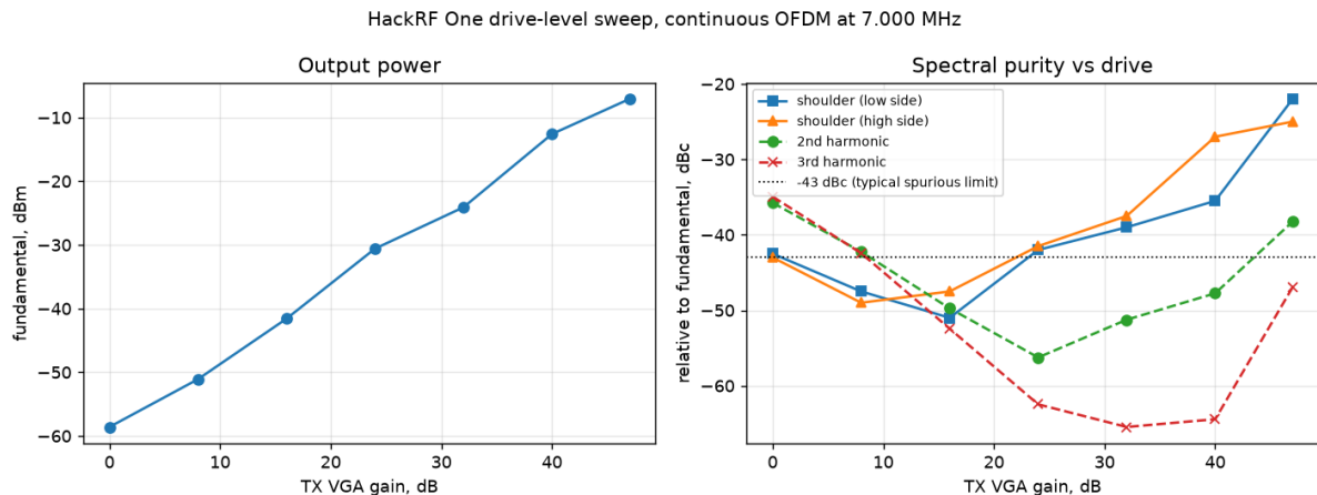
Figure 39: Drive-level sweep on the HackRF One ( demoapp/sdr_drive_sweep.py ): output power, and spectral purity relative to the fundamental, against transmit gain. Points below VGA 16 are limited by the analyser’s noise floor, not by the transmitter.
