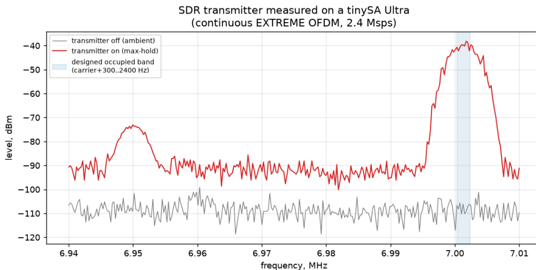
Figure 38: The transmitter measured on a tinySA Ultra: continuous EXTREME OFDM at 2.4 Msps, carrier 7.000 MHz, 3 kHz RBW. The shaded band is the designed occupancy (carrier + 300...2400 Hz); the spur at 6.95 MHz is the offset-tuned local oscillator.
