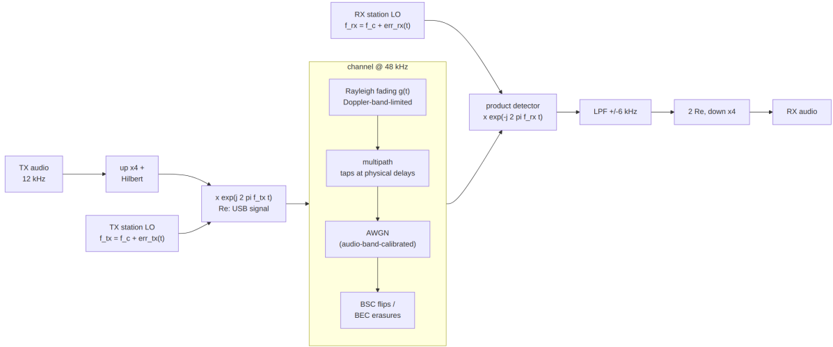
Figure 26: The RF chain: USB modulator, 48 kHz channel (fading, multipath, AWGN, BSC/BEC), product detector.
