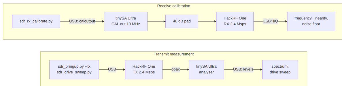
Figure 43: Instrumented bench, both directions: as an analyser the tinySA measures what the radio transmits; as a source its calibration output drives the receiver through a 40 dB pad.
