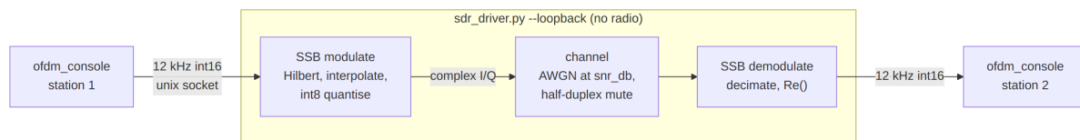
Figure 42: Hardware-free loopback: two stations cross-connected through the full SSB modulation and demodulation chain.
