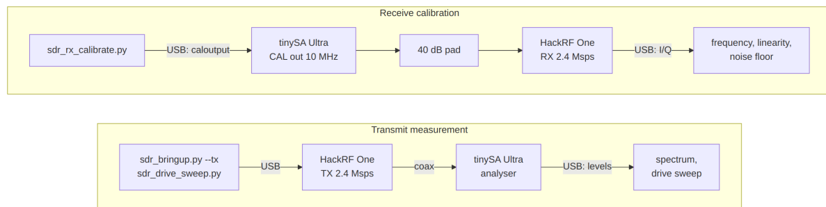
Figure 44: Instrumented bench, both directions: as an analyser the tinySA measures what the radio transmits; as a source its calibration output drives the receiver through a 40 dB pad.
