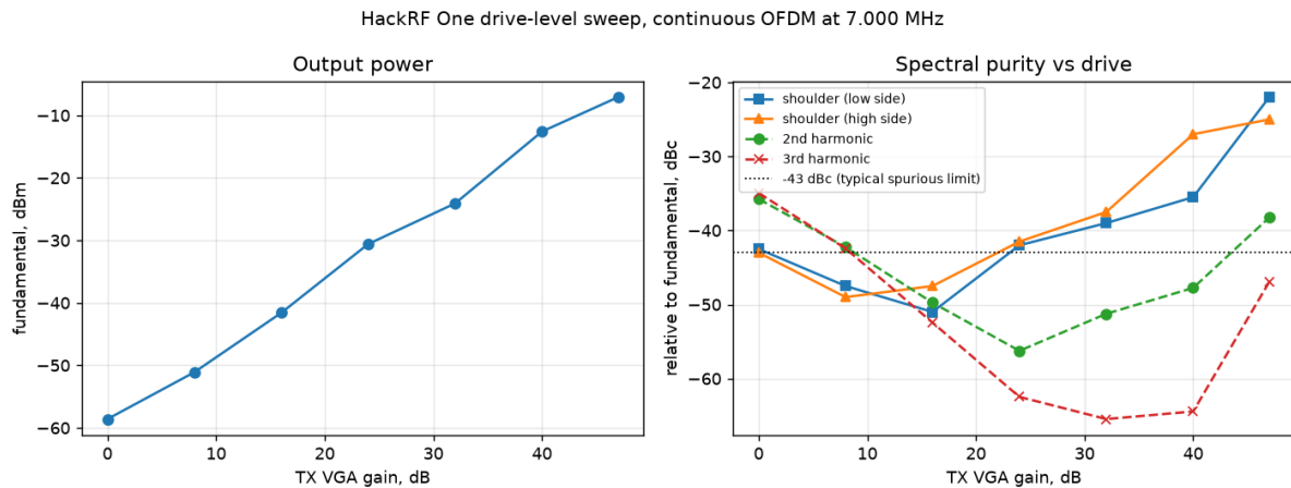
Figure 46: Drive-level sweep on the HackRF One ( demoapp/sdr_drive_sweep.py ): output power, and spectral purity relative to the fundamental, against transmit gain. Points below VGA 16 are limited by the analyser’s noise floor, not by the transmitter.
