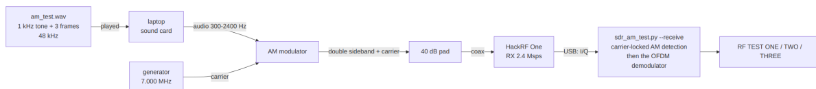
Figure 47: Off-air receive test: an external AM transmitter feeds the SDR through a 40 dB pad.
