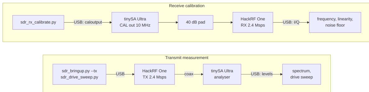
Figure 47: Instrumented bench, both directions: as an analyser the tinySA measures what the radio transmits; as a source its calibration output drives the receiver through a 40 dB pad.
