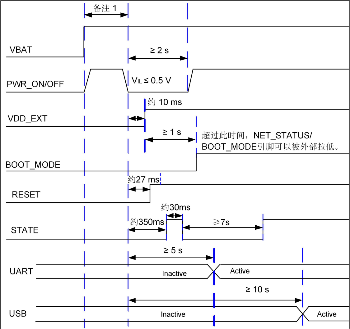
Figure 12. 开机时序图
