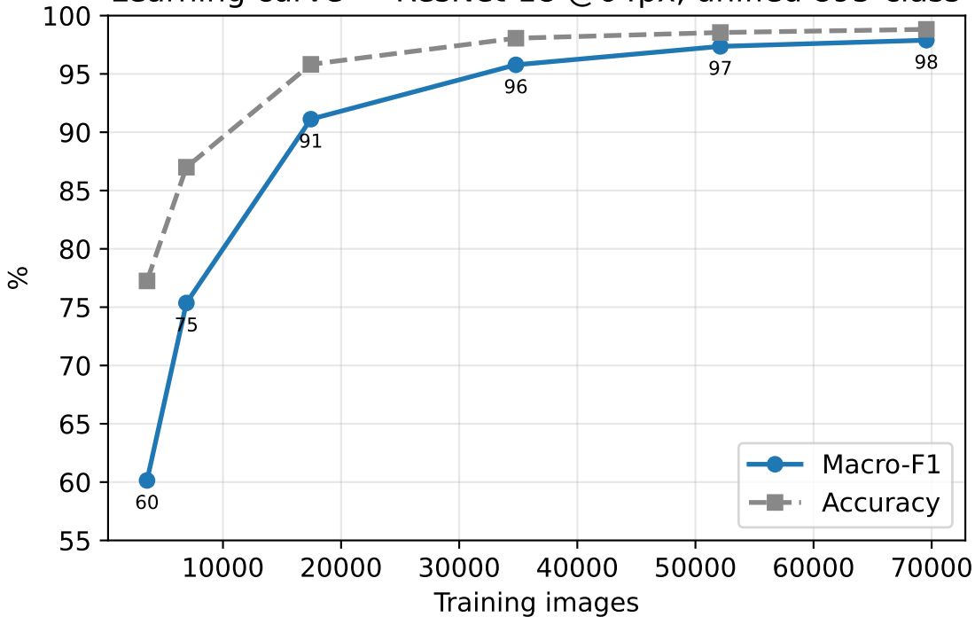
Learning curve — ResNet-18 @64px, unified 895-class
