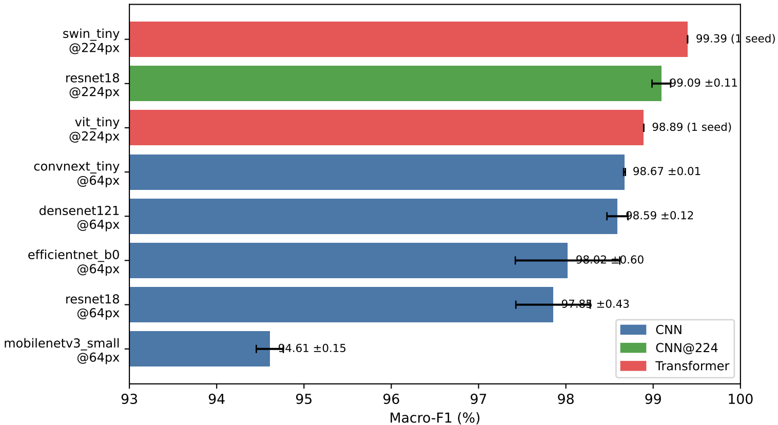
Backbone comparison - unified 895-class task
