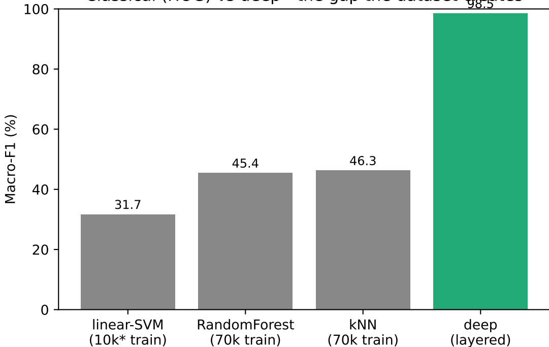
Classical (HOG) vs deep - the gap the dataset creates
