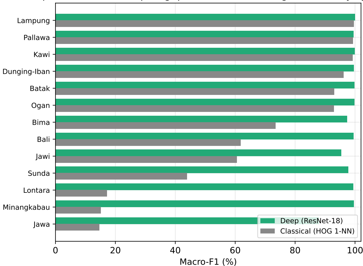
Per-script: classical vs deep — gap concentrated in high-cardinality syllabaries
