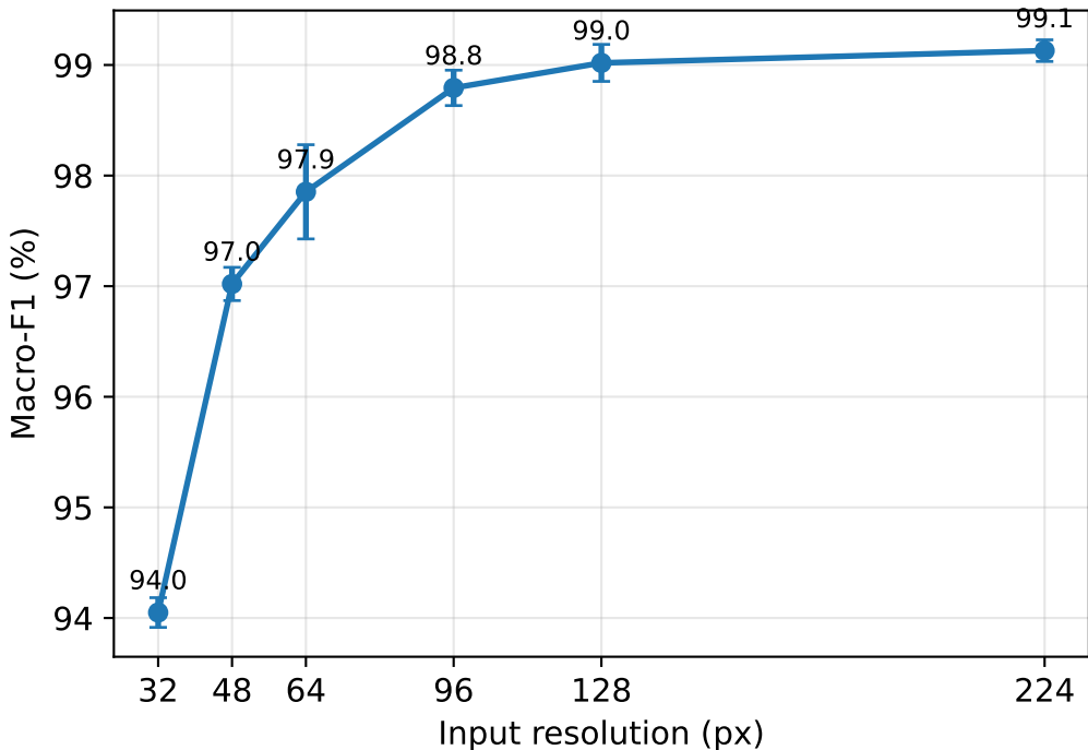
ResNet-18, unified 895-class (mean \pm std, 3 seeds)
