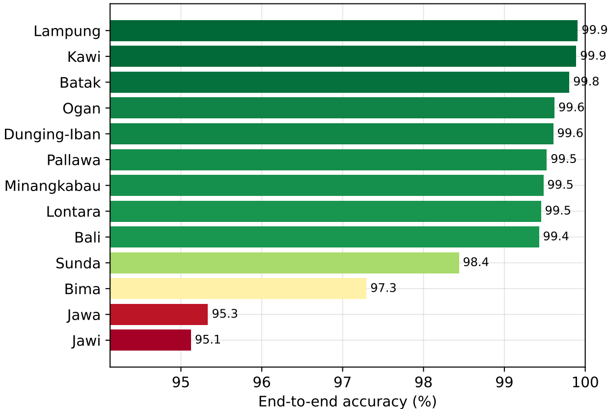
Per-script end-to-end accuracy (mean, 3 seeds)
