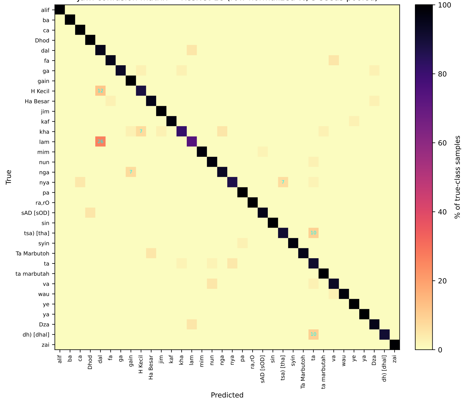
Jawi confusion matrix — ResNet-18 (row-normalized %, 3 seeds pooled)
