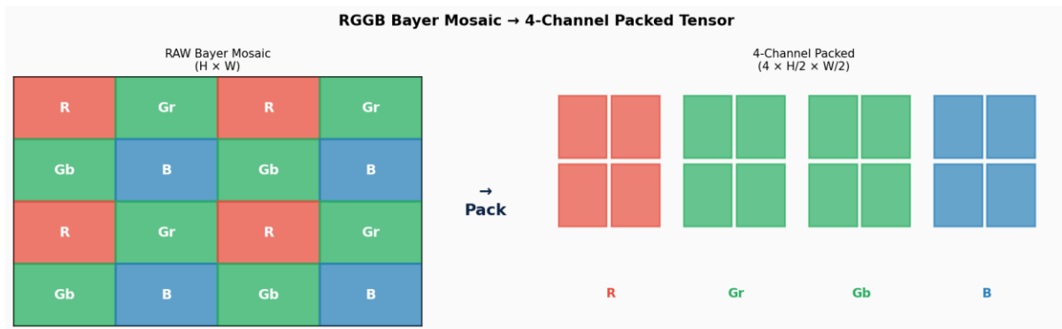
Figure 1: RGGB Bayer mosaic decomposed into 4 separate channel arrays of size H/2 \times W/2 .
