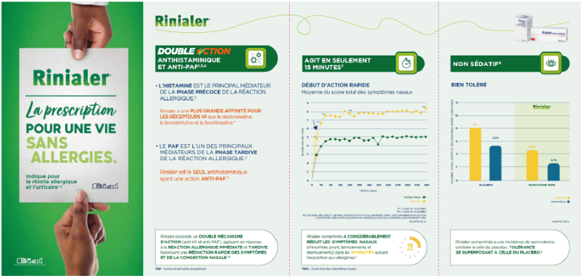
Plaquette
