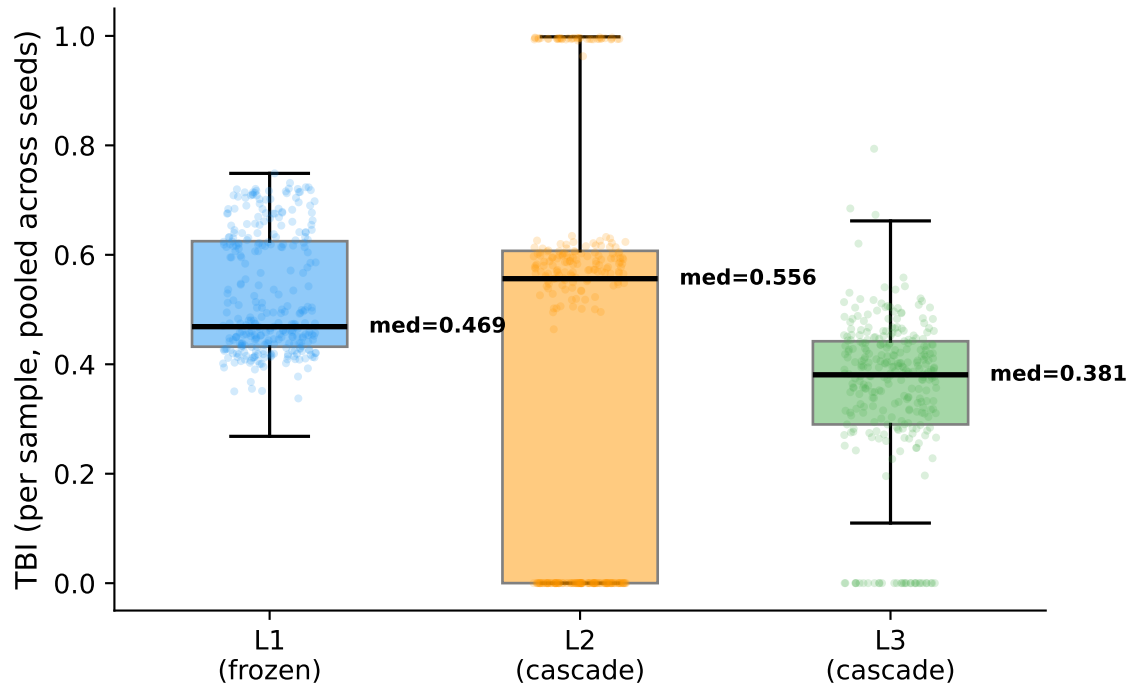
(a) Per-sample TBI distributions (5 seeds × 1280 samples each)
