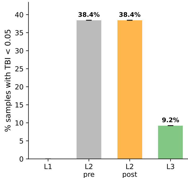
(b) Zero-coherence mode (mean \pm SD across 5 seeds)
