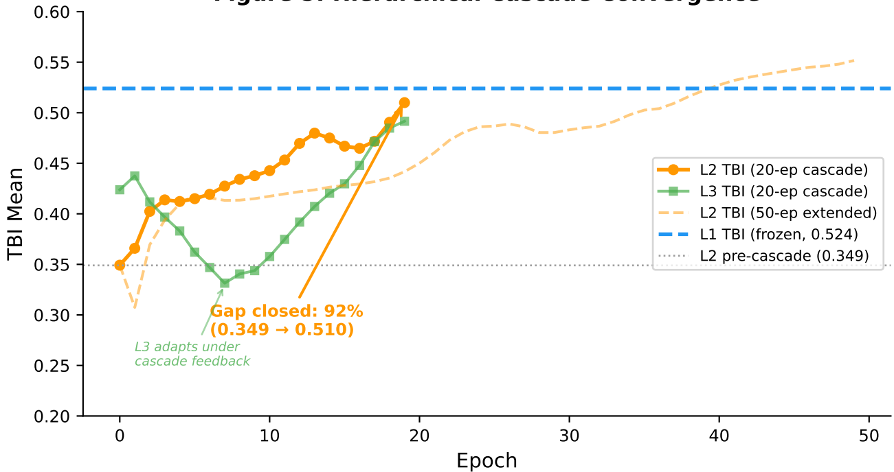
Figure 5: Hierarchical Cascade Convergence
