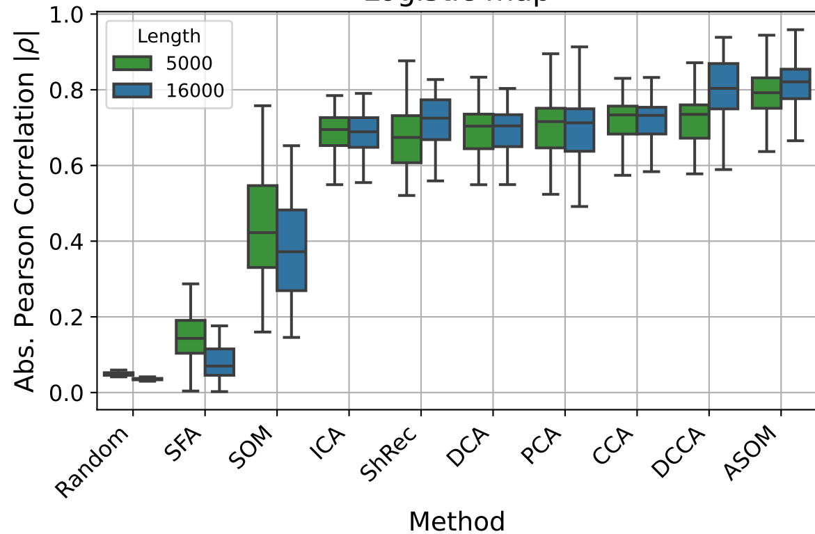
Logistic map
