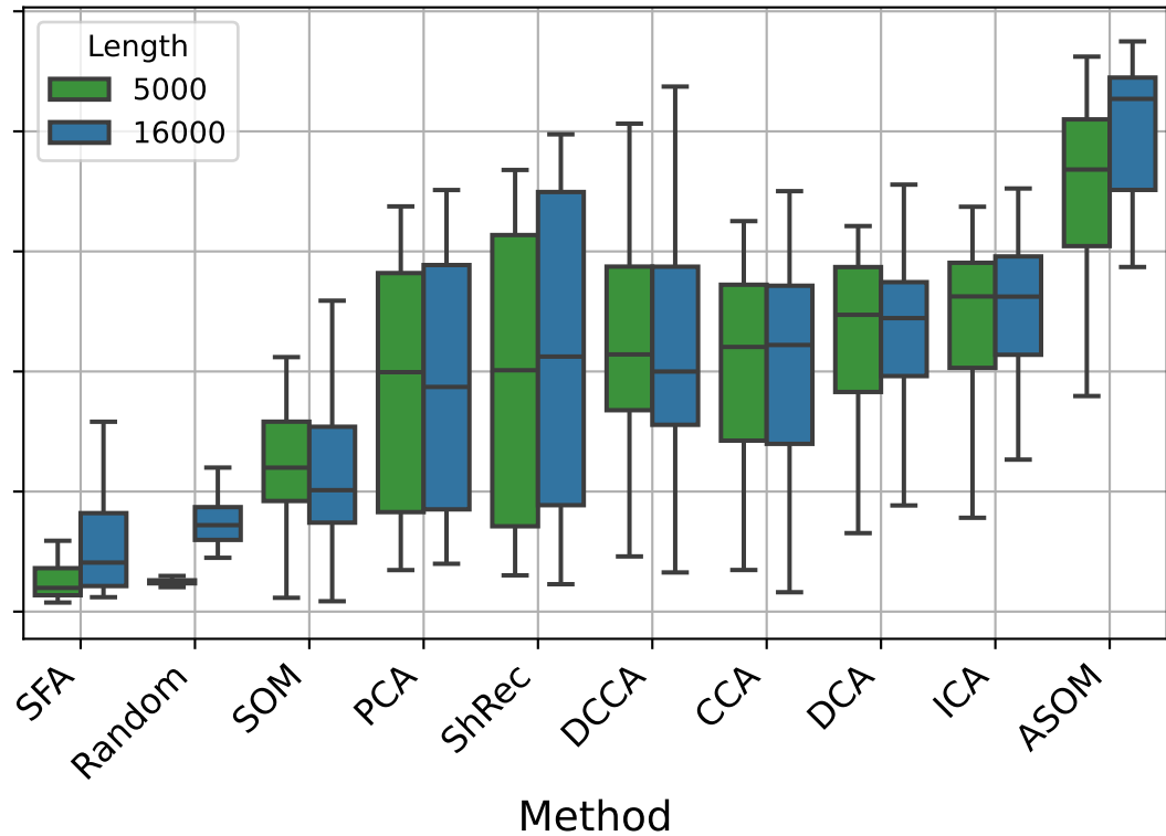
Tent map
