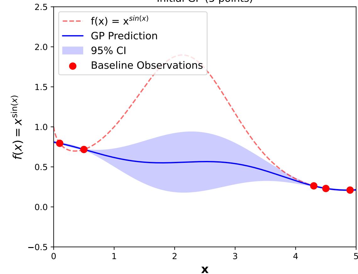
Initial GP (5 points)
