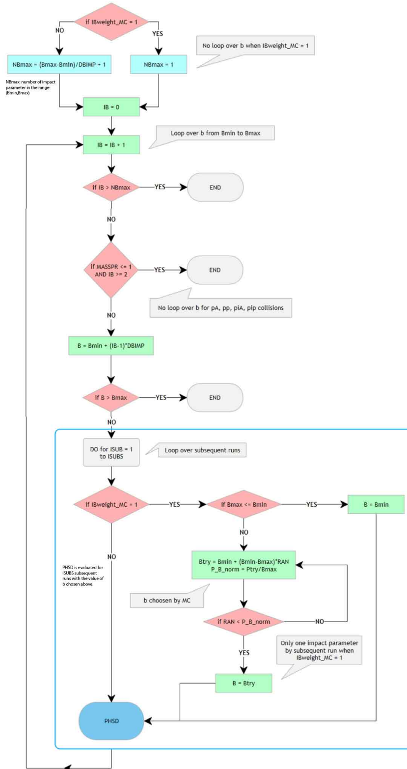
FIG. 2.3: Algorithm showing the two different options for the choice in impact parameter. For IBweightMC=1 the impact parameter is chosen by Monte Carlo according to the Min. Bias probability. For IBweightMC=0 it is simply chosen with a constant probability from a range (b_{min}, b_{max}) with a step DBIMP .
