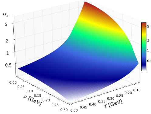
FIG. 4.2: Coupling constant \alpha_s = \frac{g^2}{4\pi} in the Dynamical QuasiParticle Model.
