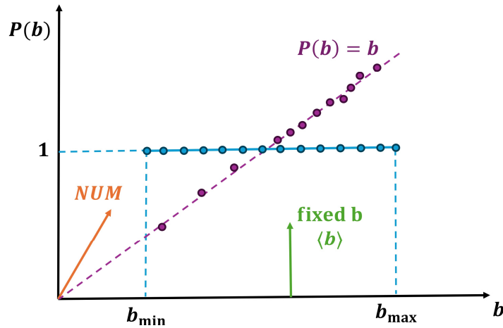
FIG. 2.1: Probability distribution P(b) as a function of the impact parameter b in PHSD–PHQMD. One can use a fixed impact parameter, or a range (b_{\min}, b_{\max}) , or the minimum bias distribution (see text for explanations).
